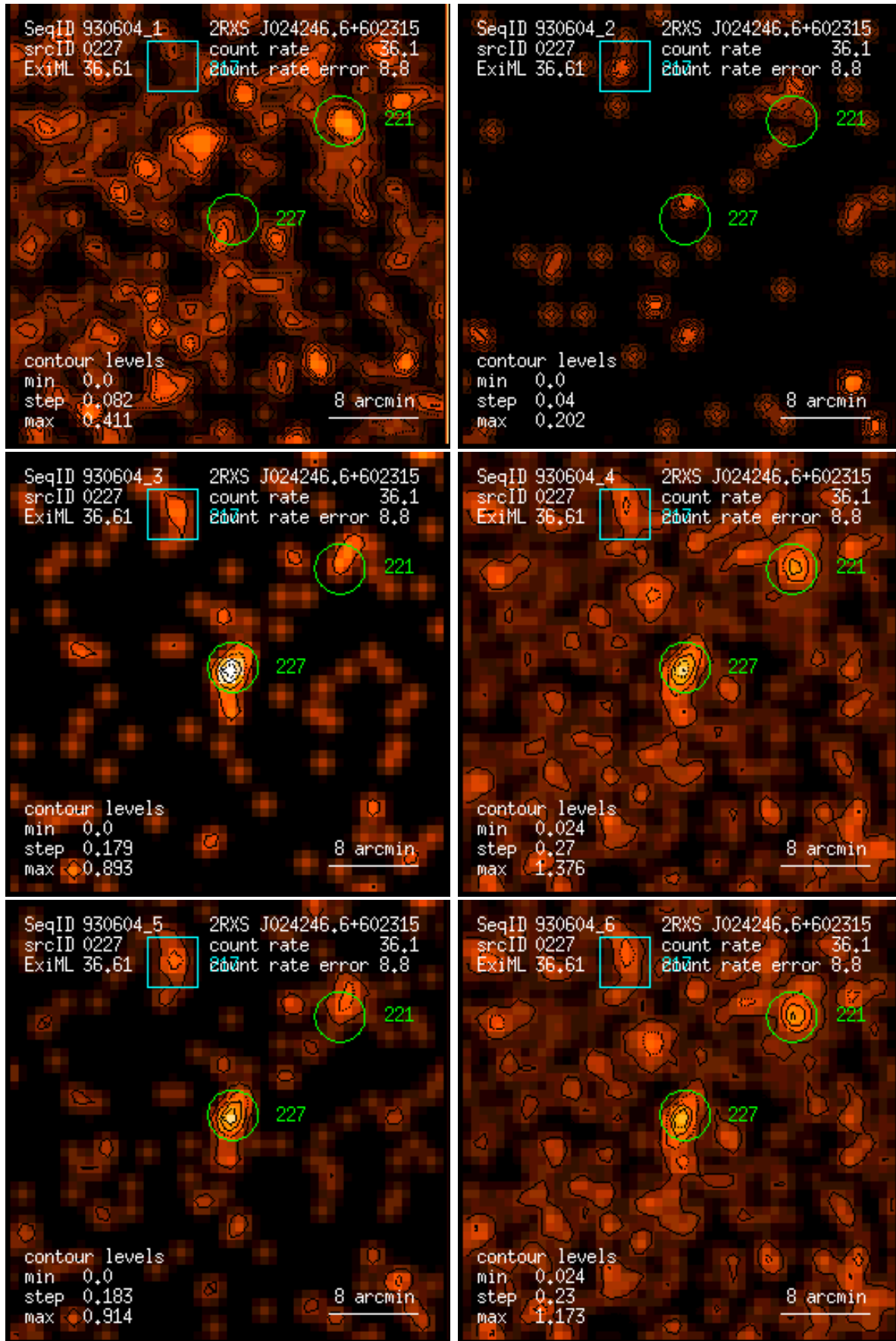
Figure 227: RASS 930604: detection 0227: band rate images, Gaussian filter: (1) PSPC channels 11 – 41, (2) 52 – 90, (3) 91 – 201, (4) 11 – 235, (5) 52 – 201, (6) 11 – 201. Broad band rates in counts/ks. Band rate contour levels in counts/ks/arcmin 2 .
