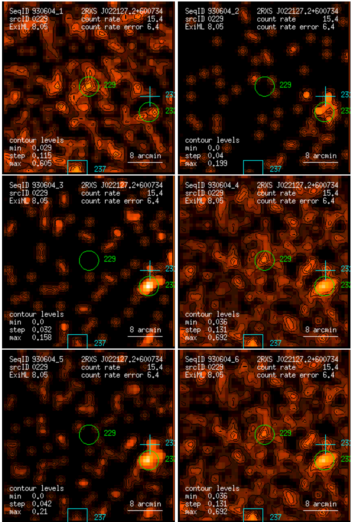
Figure 229: RASS 930604: detection 0229: band rate images, Gaussian filter: (1) PSPC channels 11 – 41, (2) 52 – 90, (3) 91 – 201, (4) 11 – 235, (5) 52 – 201, (6) 11 – 201. Broad band rates in counts/ks. Band rate contour levels in counts/ks/arcmin 2 .
