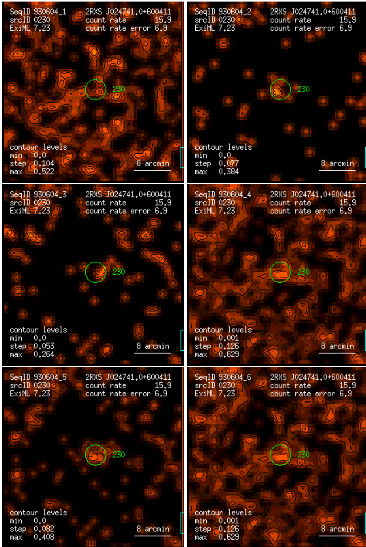
Figure 230: RASS 930604: detection 0230: band rate images, Gaussian filter: (1) PSPC channels 11 – 41, (2) 52 – 90, (3) 91 – 201, (4) 11 – 235, (5) 52 – 201, (6) 11 – 201. Broad band rates in counts/ks. Band rate contour levels in counts/ks/arcmin 2 .
