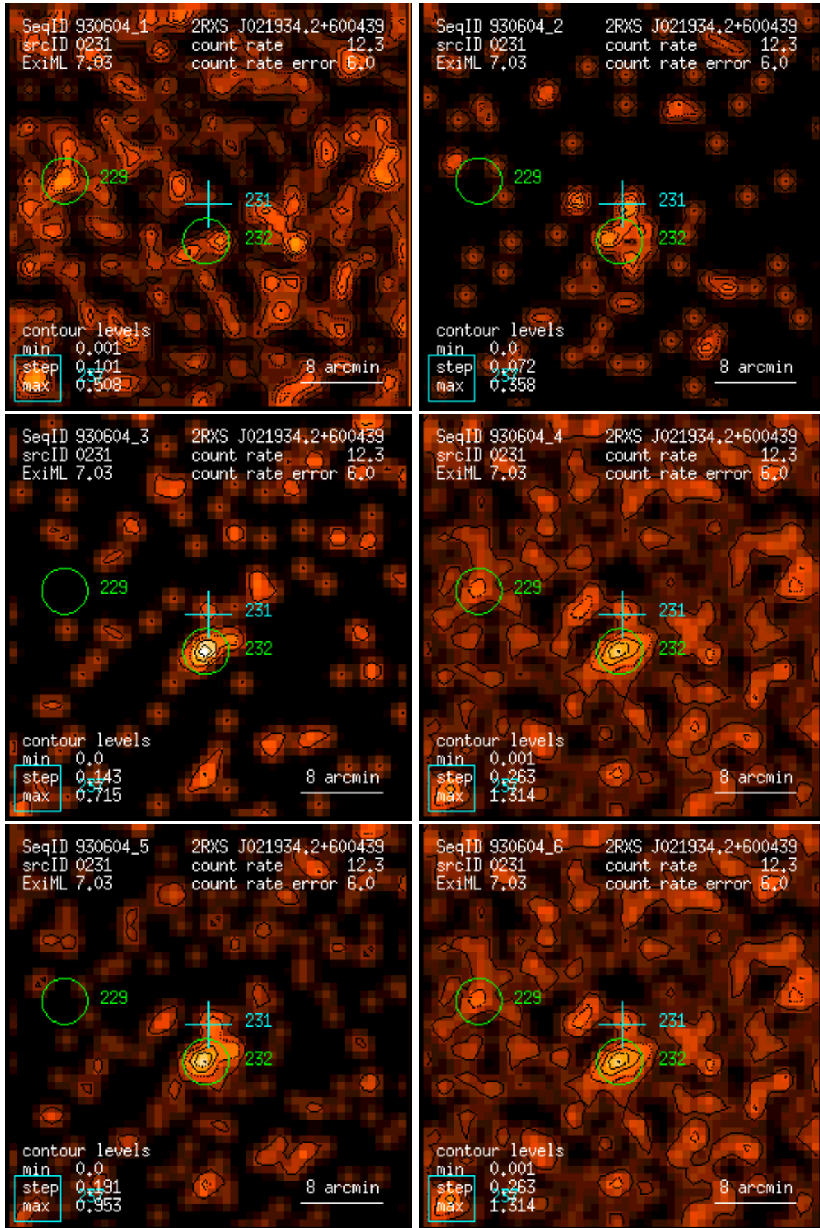
Figure 231: RASS 930604: detection 0231: band rate images, Gaussian filter: (1) PSPC channels 11 – 41, (2) 52 – 90, (3) 91 – 201, (4) 11 – 235, (5) 52 – 201, (6) 11 – 201. Broad band rates in counts/ks. Band rate contour levels in counts/ks/arcmin 2 .
