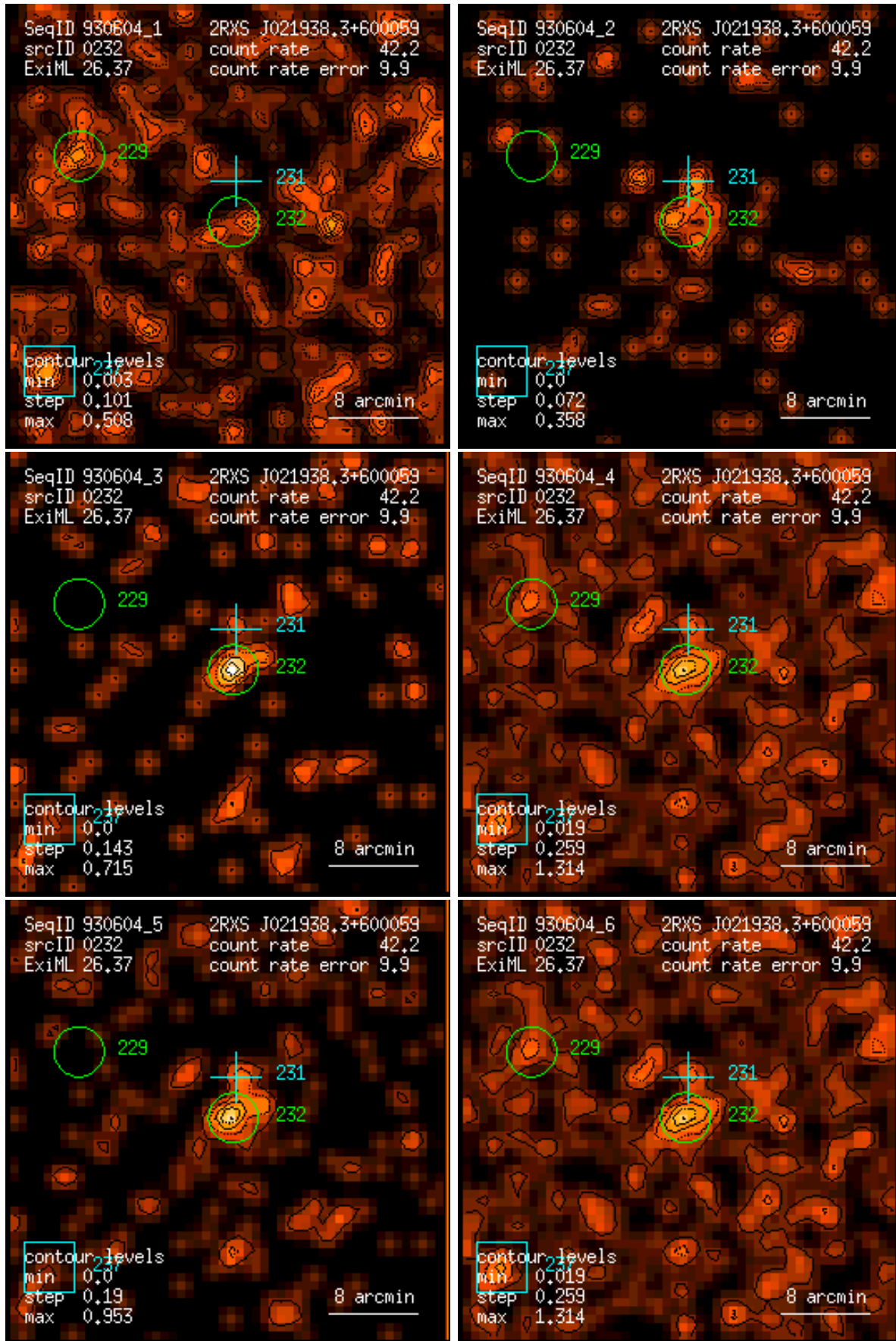
Figure 232: RASS 930604: detection 0232: band rate images, Gaussian filter: (1) PSPC channels 11 – 41, (2) 52 – 90, (3) 91 – 201, (4) 11 – 235, (5) 52 – 201, (6) 11 – 201. Broad band rates in counts/ks. Band rate contour levels in counts/ks/arcmin 2 .
