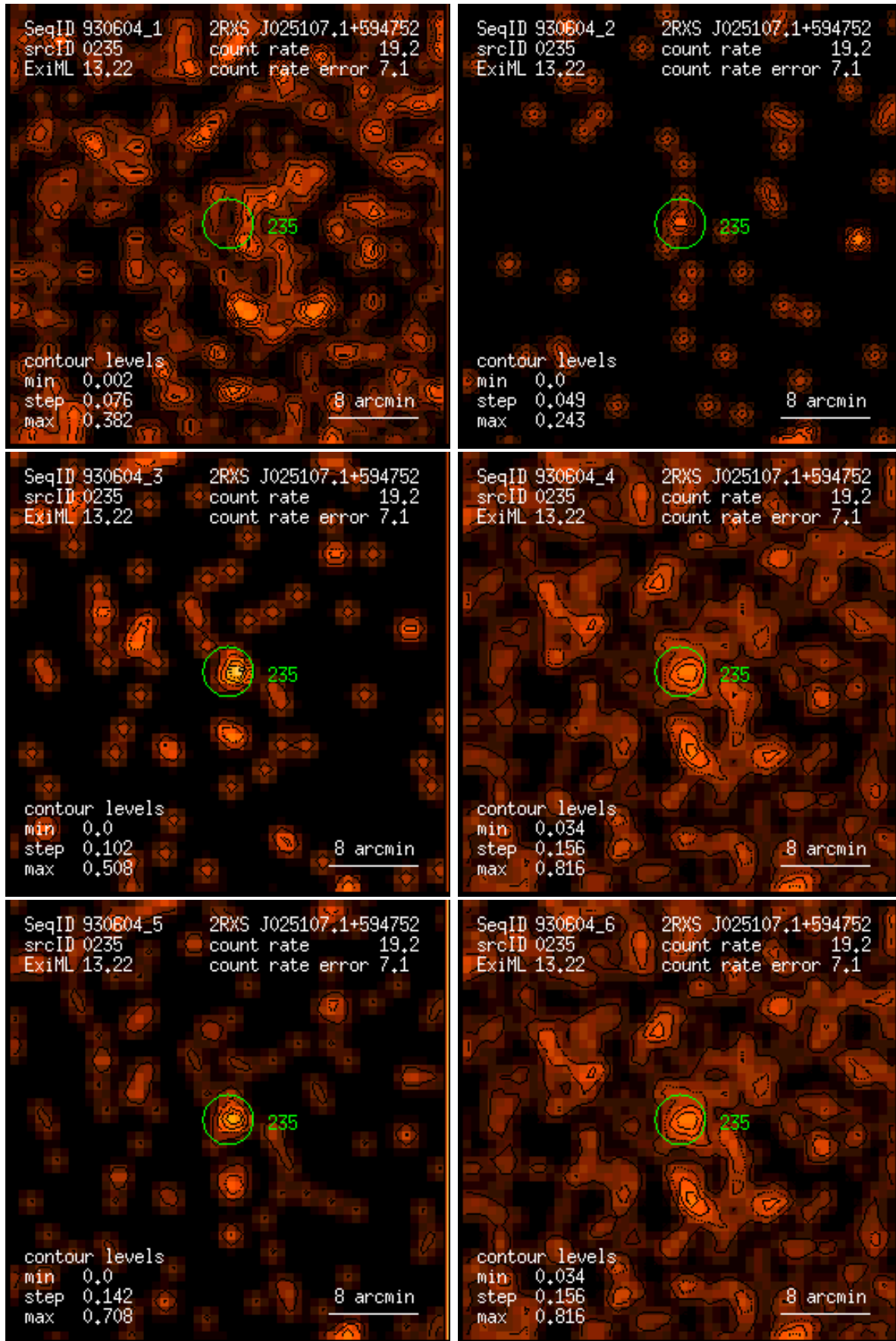
Figure 235: RASS 930604: detection 0235: band rate images, Gaussian filter: (1) PSPC channels 11 – 41, (2) 52 – 90, (3) 91 – 201, (4) 11 – 235, (5) 52 – 201, (6) 11 – 201. Broad band rates in counts/ks. Band rate contour levels in counts/ks/arcmin 2 .
