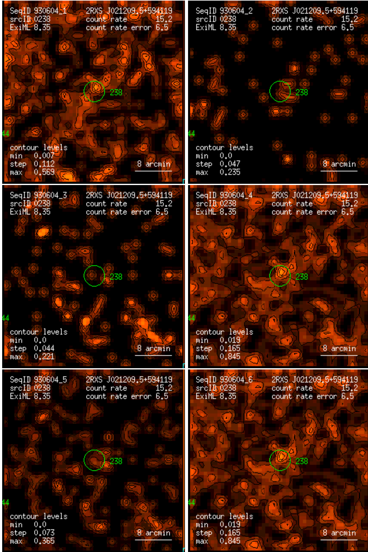
Figure 238: RASS 930604: detection 0238: band rate images, Gaussian filter: (1) PSPC channels 11 – 41, (2) 52 – 90, (3) 91 – 201, (4) 11 – 235, (5) 52 – 201, (6) 11 – 201. Broad band rates in counts/ks. Band rate contour levels in counts/ks/arcmin 2 .
