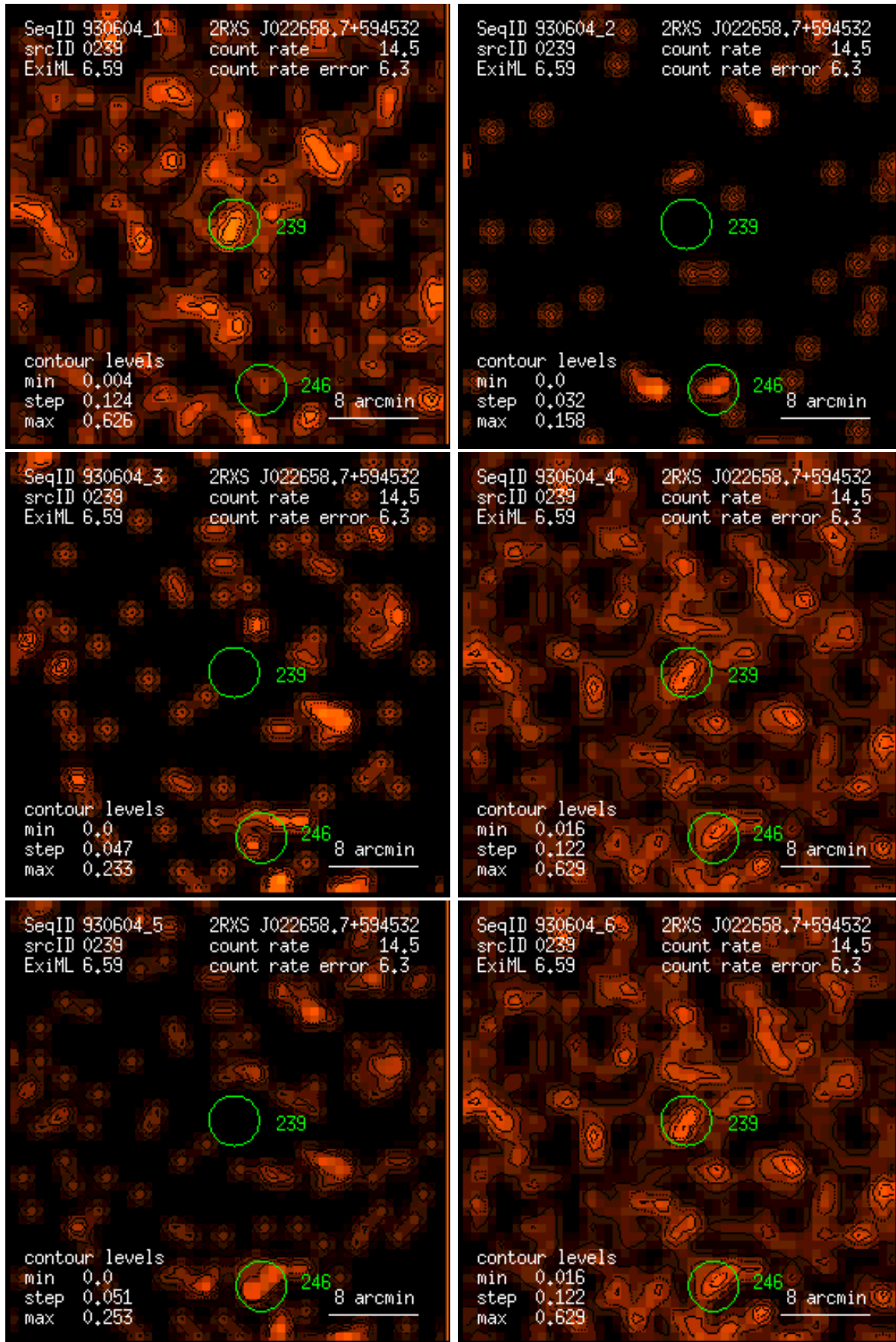
Figure 239: RASS 930604: detection 0239: band rate images, Gaussian filter: (1) PSPC channels 11 – 41, (2) 52 – 90, (3) 91 – 201, (4) 11 – 235, (5) 52 – 201, (6) 11 – 201. Broad band rates in counts/ks. Band rate contour levels in counts/ks/arcmin 2 .
