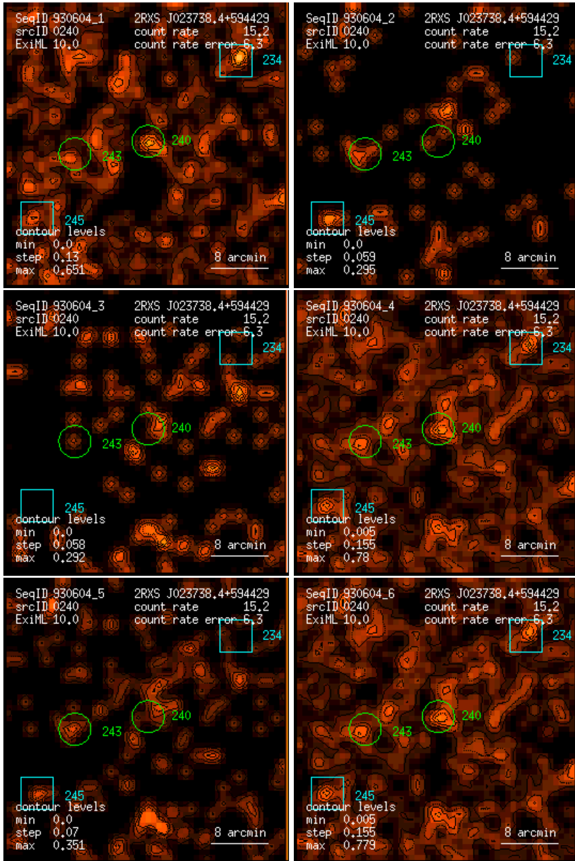
Figure 240: RASS 930604: detection 0240: band rate images, Gaussian filter: (1) PSPC channels 11 – 41, (2) 52 – 90, (3) 91 – 201, (4) 11 – 235, (5) 52 – 201, (6) 11 – 201. Broad band rates in counts/ks. Band rate contour levels in counts/ks/arcmin 2 .
