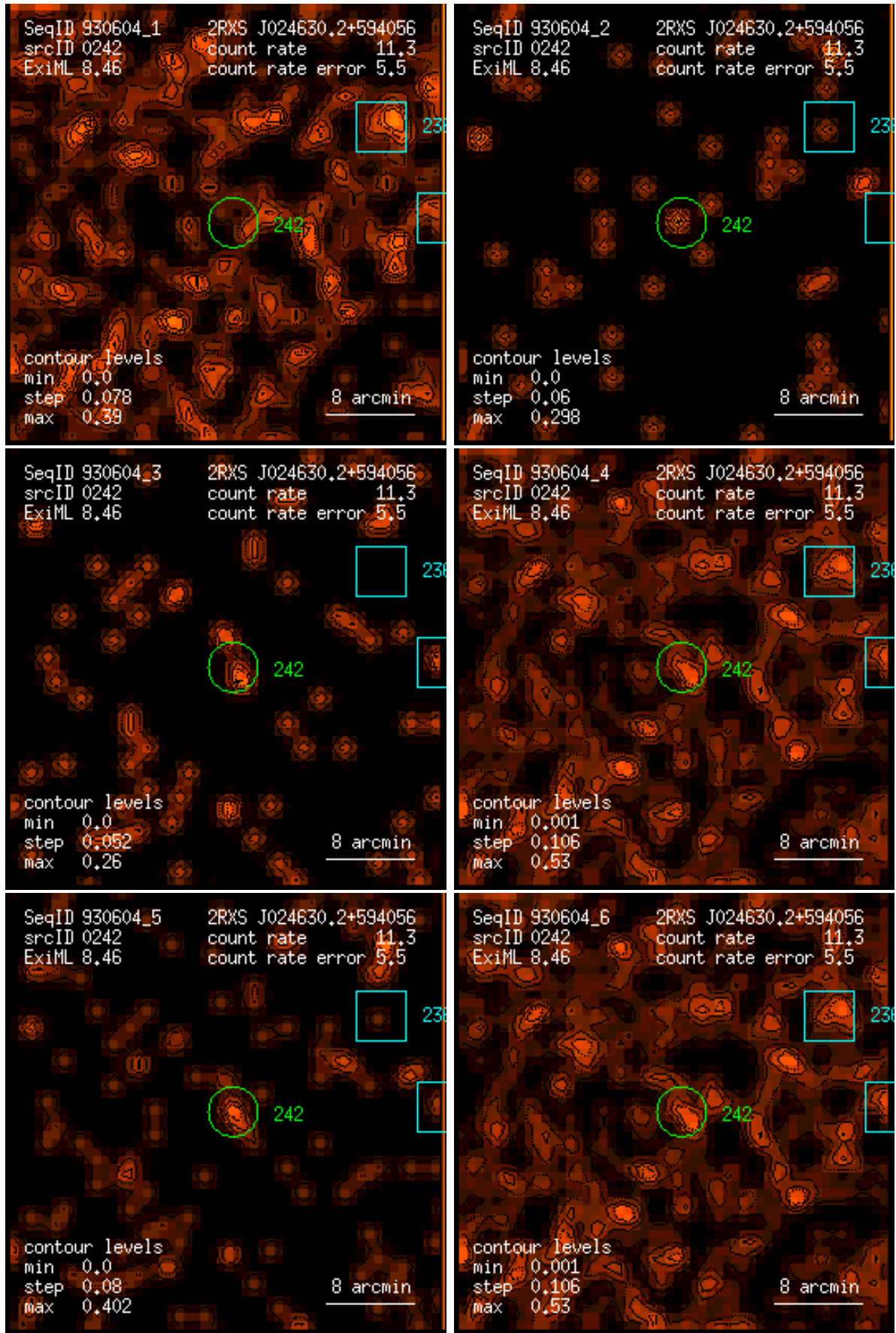
Figure 242: RASS 930604: detection 0242: band rate images, Gaussian filter: (1) PSPC channels 11 – 41, (2) 52 – 90, (3) 91 – 201, (4) 11 – 235, (5) 52 – 201, (6) 11 – 201. Broad band rates in counts/ks. Band rate contour levels in counts/ks/arcmin 2 .
