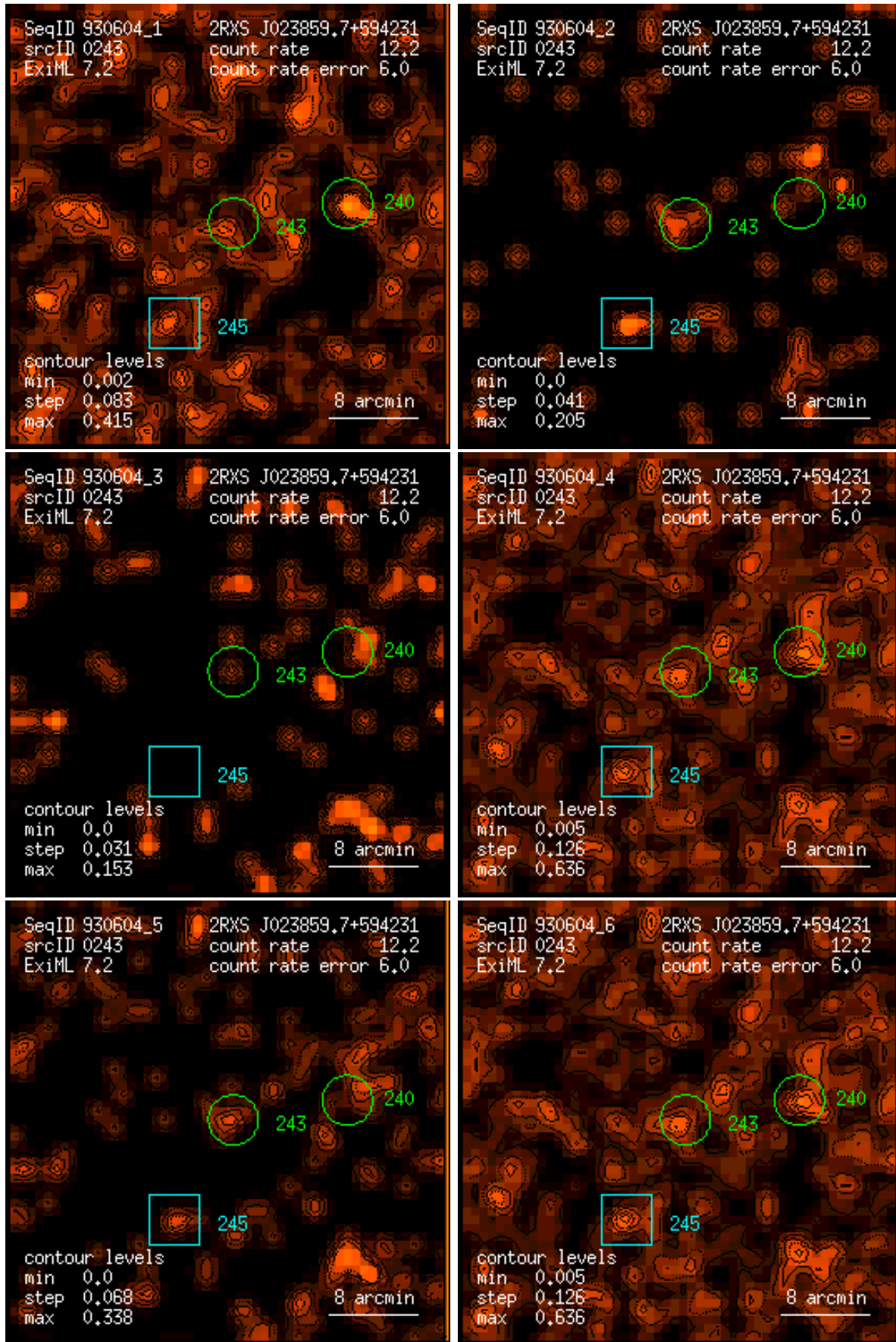
Figure 243: RASS 930604: detection 0243: band rate images, Gaussian filter: (1) PSPC channels 11 – 41, (2) 52 – 90, (3) 91 – 201, (4) 11 – 235, (5) 52 – 201, (6) 11 – 201. Broad band rates in counts/ks. Band rate contour levels in counts/ks/arcmin 2 .
