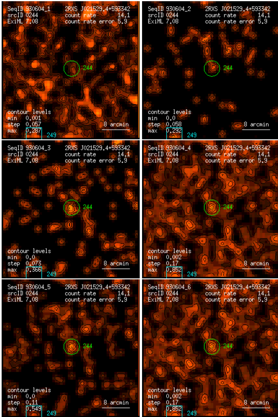
Figure 244: RASS 930604: detection 0244: band rate images, Gaussian filter: (1) PSPC channels 11 – 41, (2) 52 – 90, (3) 91 – 201, (4) 11 – 235, (5) 52 – 201, (6) 11 – 201. Broad band rates in counts/ks. Band rate contour levels in counts/ks/arcmin 2 .
