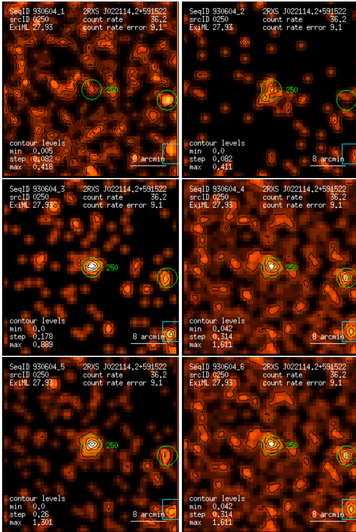
Figure 250: RASS 930604: detection 0250: band rate images, Gaussian filter: (1) PSPC channels 11 – 41, (2) 52 – 90, (3) 91 – 201, (4) 11 – 235, (5) 52 – 201, (6) 11 – 201. Broad band rates in counts/ks. Band rate contour levels in counts/ks/arcmin 2 .
