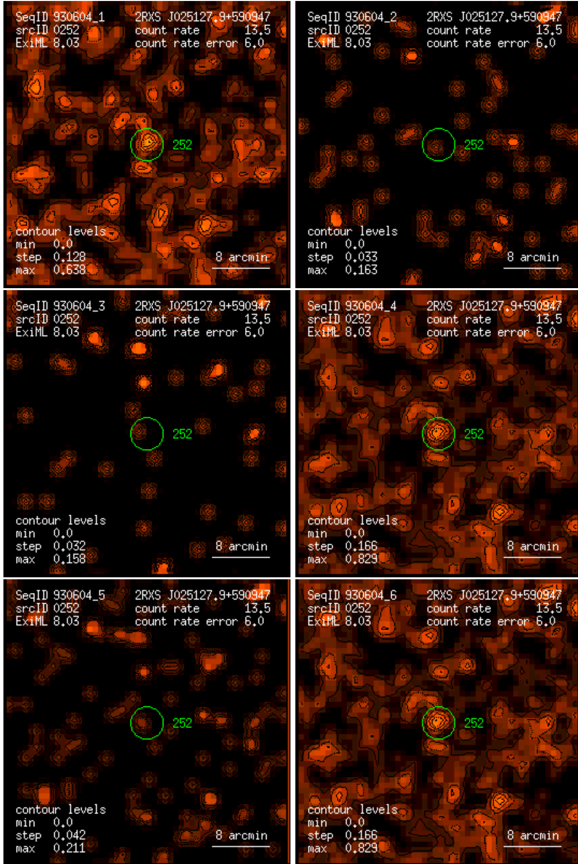
Figure 252: RASS 930604: detection 0252: band rate images, Gaussian filter: (1) PSPC channels 11 – 41, (2) 52 – 90, (3) 91 – 201, (4) 11 – 235, (5) 52 – 201, (6) 11 – 201. Broad band rates in counts/ks. Band rate contour levels in counts/ks/arcmin 2 .
