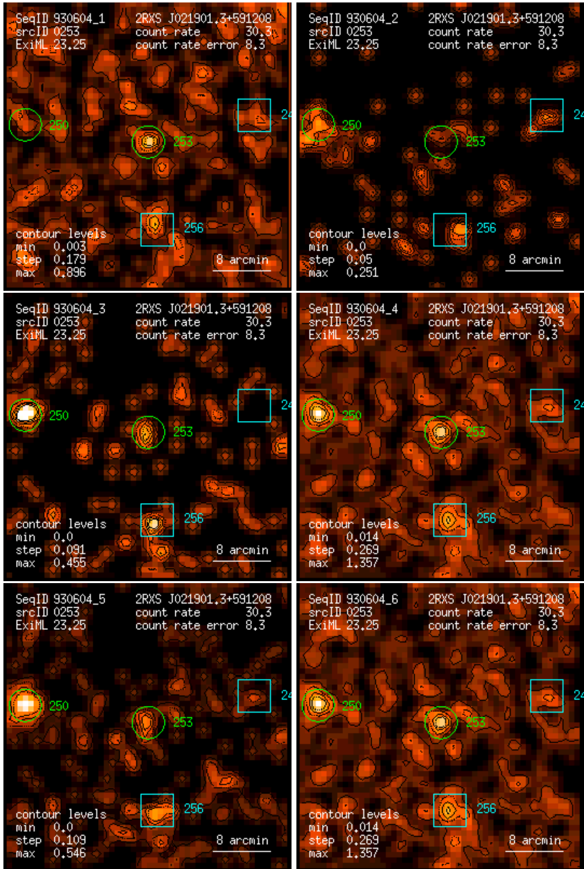
Figure 253: RASS 930604: detection 0253: band rate images, Gaussian filter: (1) PSPC channels 11 – 41, (2) 52 – 90, (3) 91 – 201, (4) 11 – 235, (5) 52 – 201, (6) 11 – 201. Broad band rates in counts/ks. Band rate contour levels in counts/ks/arcmin 2 .
