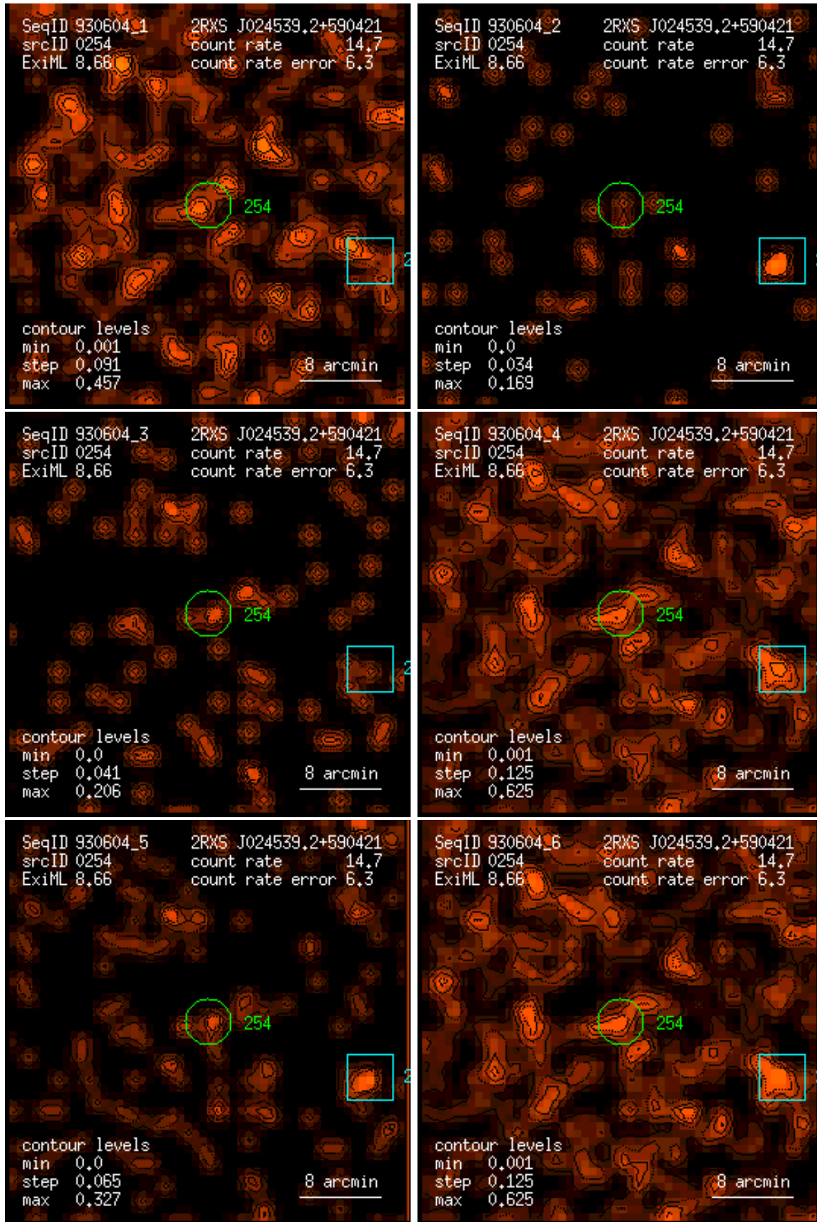
Figure 254: RASS 930604: detection 0254: band rate images, Gaussian filter: (1) PSPC channels 11 – 41, (2) 52 – 90, (3) 91 – 201, (4) 11 – 235, (5) 52 – 201, (6) 11 – 201. Broad band rates in counts/ks. Band rate contour levels in counts/ks/arcmin 2 .
