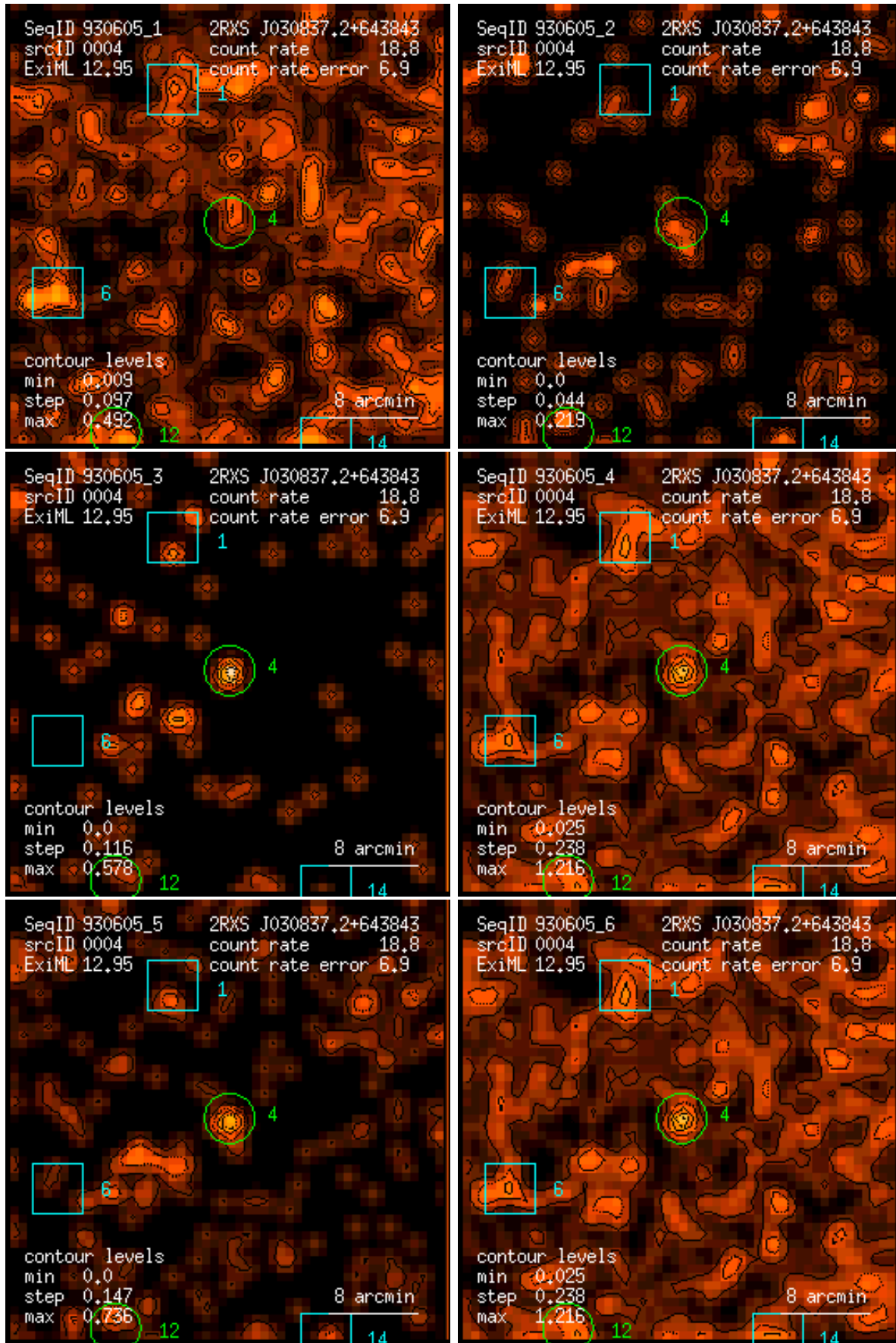
Figure 4: RASS 930605: detection 0004: band rate images, Gaussian filter: (1) PSPC channels 11 – 41, (2) 52 – 90, (3) 91 – 201, (4) 11 – 235, (5) 52 – 201, (6) 11 – 201. Broad band rates in counts/ks. Band rate contour levels in counts/ks/arcmin 2 .
