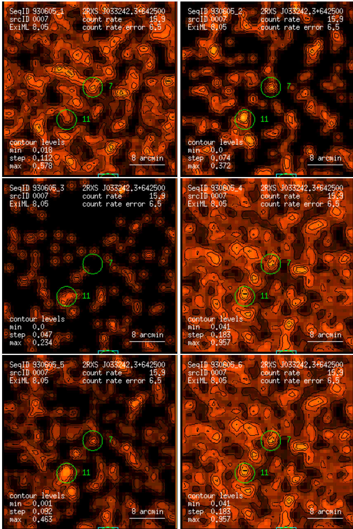
Figure 7: RASS 930605: detection 0007: band rate images, Gaussian filter: (1) PSPC channels 11 – 41, (2) 52 – 90, (3) 91 – 201, (4) 11 – 235, (5) 52 – 201, (6) 11 – 201. Broad band rates in counts/ks. Band rate contour levels in counts/ks/arcmin 2 .
