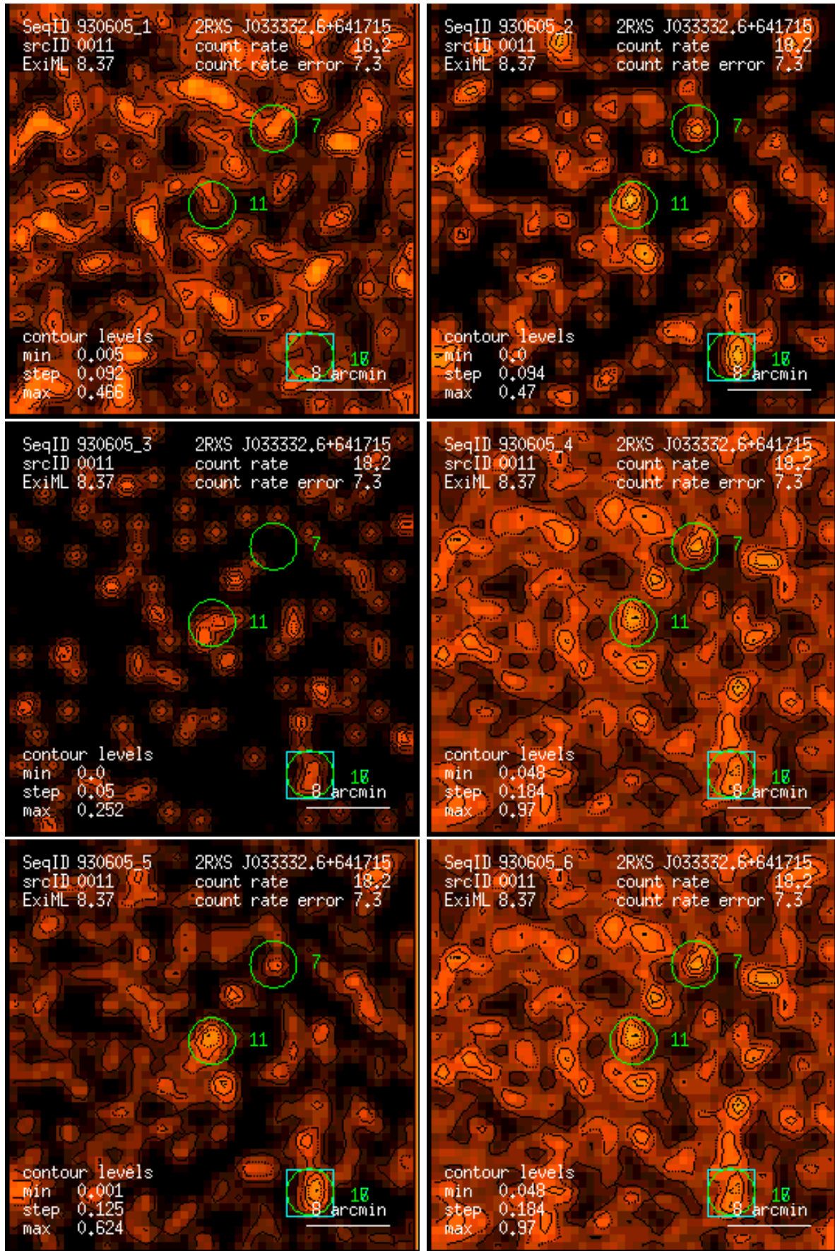
Figure 11: RASS 930605: detection 0011: band rate images, Gaussian filter: (1) PSPC channels 11 – 41, (2) 52 – 90, (3) 91 – 201, (4) 11 – 235, (5) 52 – 201, (6) 11 – 201. Broad band rates in counts/ks. Band rate contour levels in counts/ks/arcmin 2 .
