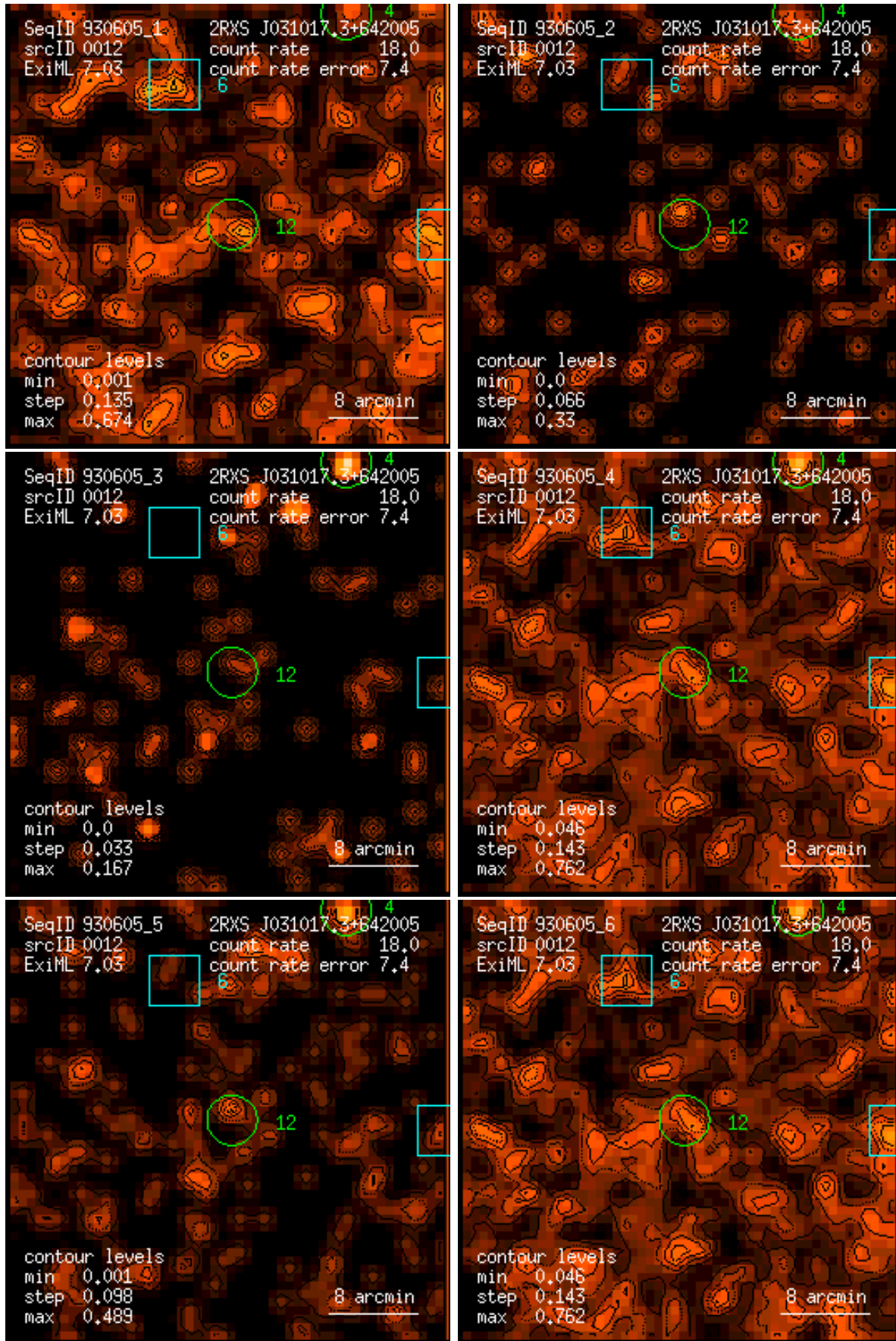
Figure 12: RASS 930605: detection 0012: band rate images, Gaussian filter: (1) PSPC channels 11 – 41, (2) 52 – 90, (3) 91 – 201, (4) 11 – 235, (5) 52 – 201, (6) 11 – 201. Broad band rates in counts/ks. Band rate contour levels in counts/ks/arcmin 2 .
