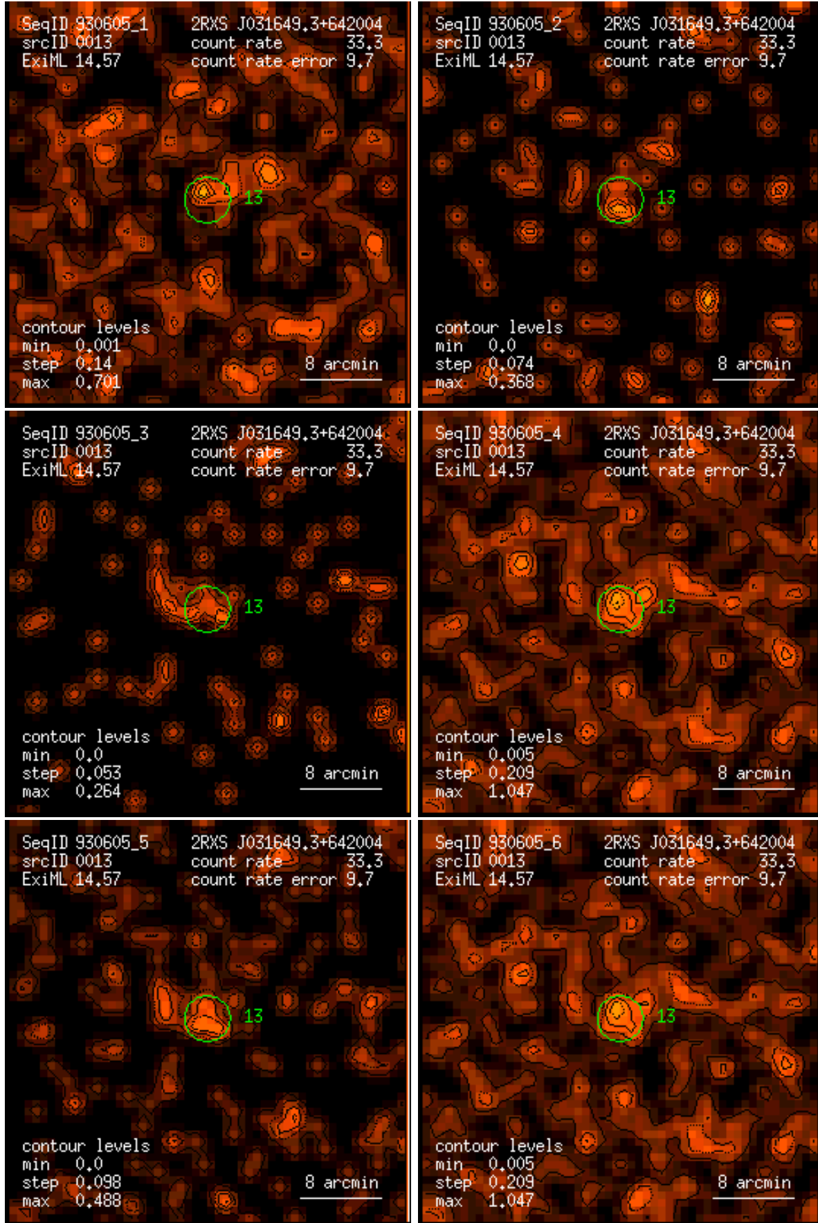
Figure 13: RASS 930605: detection 0013: band rate images, Gaussian filter: (1) PSPC channels 11 – 41, (2) 52 – 90, (3) 91 – 201, (4) 11 – 235, (5) 52 – 201, (6) 11 – 201. Broad band rates in counts/ks. Band rate contour levels in counts/ks/arcmin 2 .
