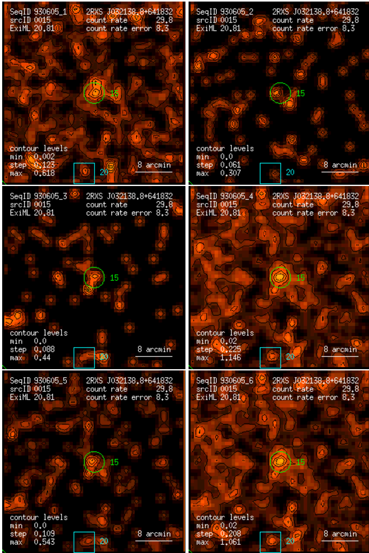
Figure 15: RASS 930605: detection 0015: band rate images, Gaussian filter: (1) PSPC channels 11 – 41, (2) 52 – 90, (3) 91 – 201, (4) 11 – 235, (5) 52 – 201, (6) 11 – 201. Broad band rates in counts/ks. Band rate contour levels in counts/ks/arcmin 2 .
