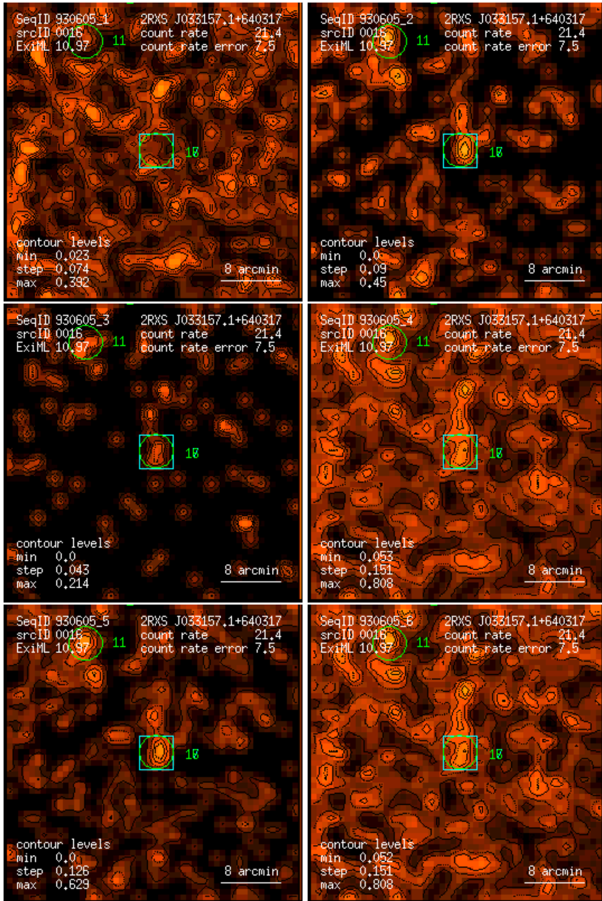
Figure 16: RASS 930605: detection 0016: band rate images, Gaussian filter: (1) PSPC channels 11 – 41, (2) 52 – 90, (3) 91 – 201, (4) 11 – 235, (5) 52 – 201, (6) 11 – 201. Broad band rates in counts/ks. Band rate contour levels in counts/ks/arcmin 2 .
