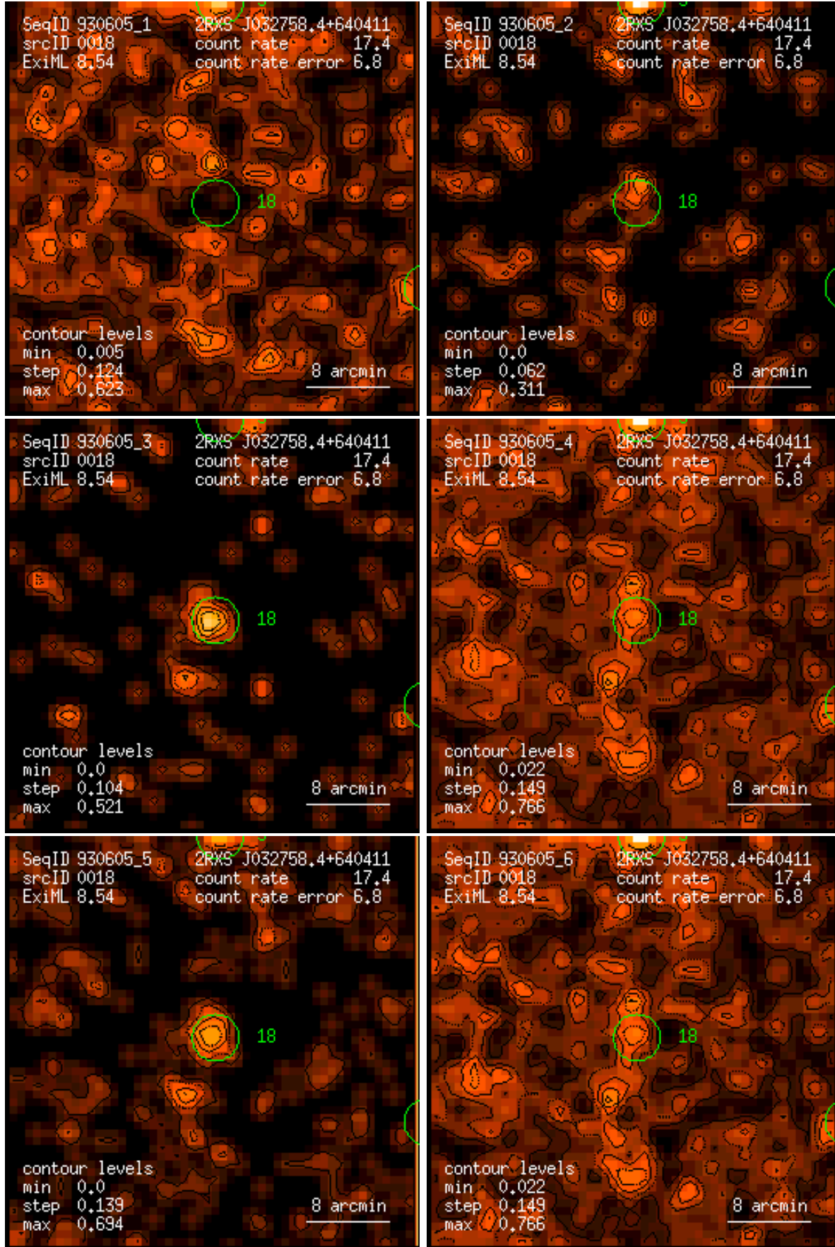
Figure 18: RASS 930605: detection 0018: band rate images, Gaussian filter: (1) PSPC channels 11 – 41, (2) 52 – 90, (3) 91 – 201, (4) 11 – 235, (5) 52 – 201, (6) 11 – 201. Broad band rates in counts/ks. Band rate contour levels in counts/ks/arcmin 2 .
