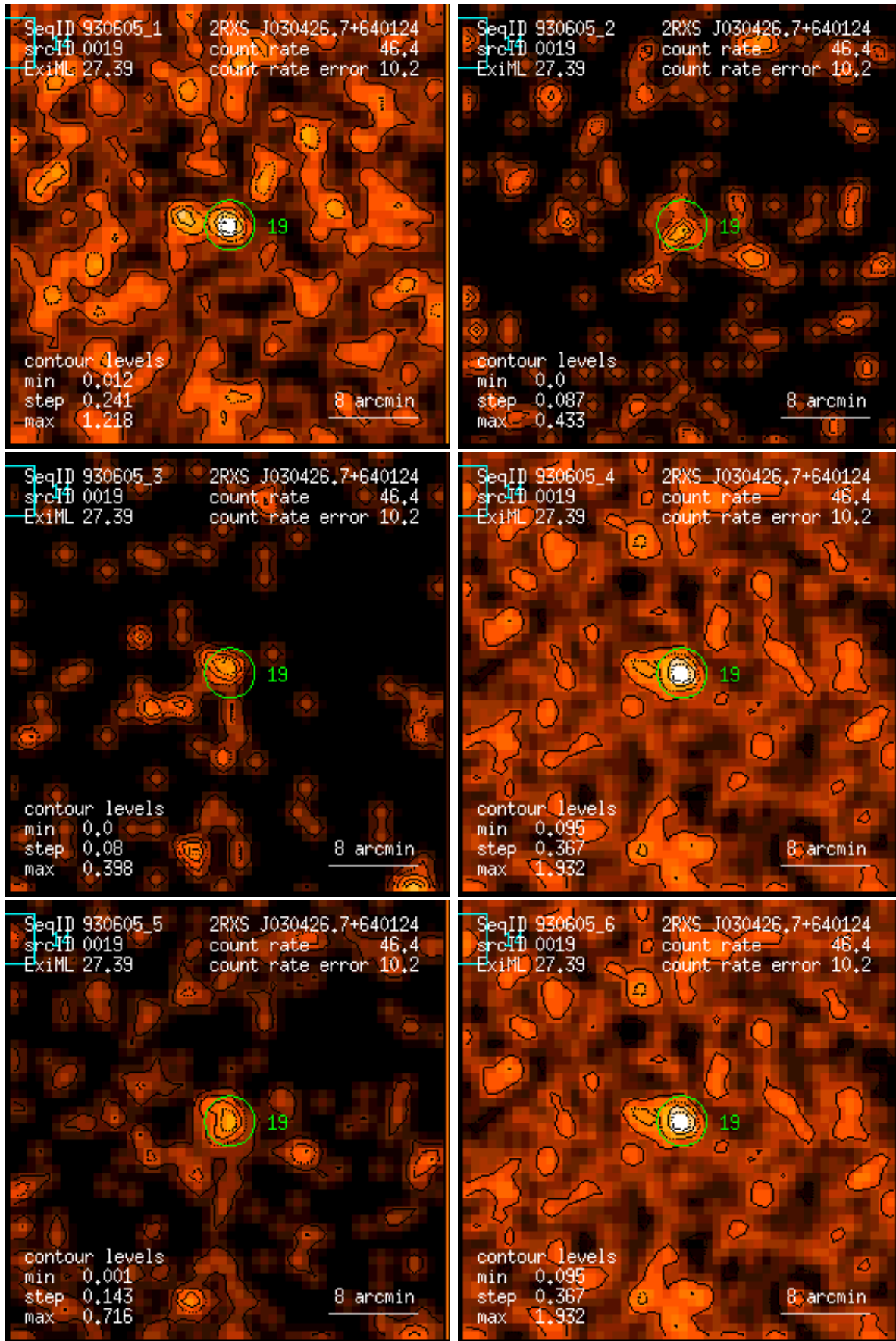
Figure 19: RASS 930605: detection 0019: band rate images, Gaussian filter: (1) PSPC channels 11 – 41, (2) 52 – 90, (3) 91 – 201, (4) 11 – 235, (5) 52 – 201, (6) 11 – 201. Broad band rates in counts/ks. Band rate contour levels in counts/ks/arcmin 2 .
