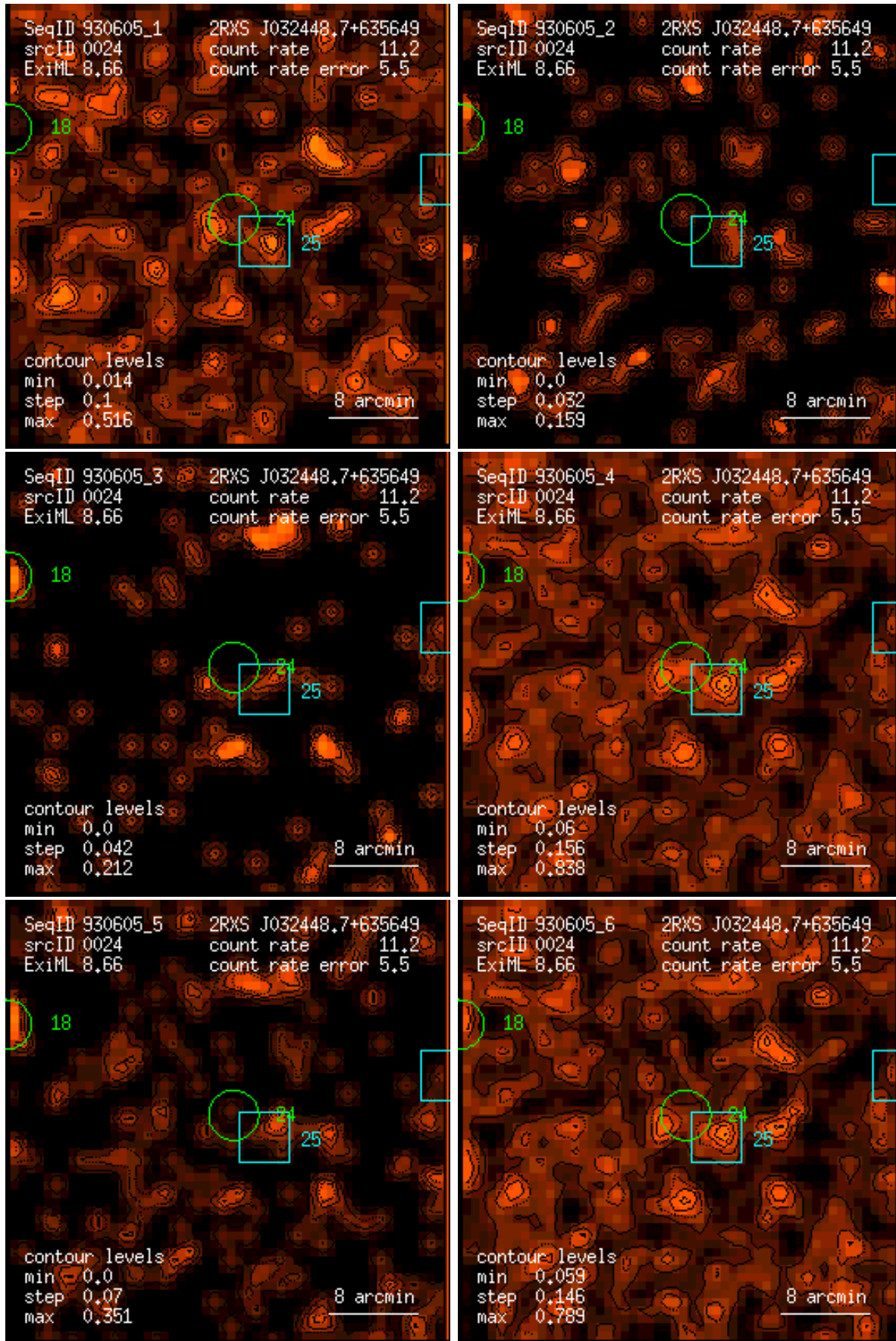
Figure 24: RASS 930605: detection 0024: band rate images, Gaussian filter: (1) PSPC channels 11 – 41, (2) 52 – 90, (3) 91 – 201, (4) 11 – 235, (5) 52 – 201, (6) 11 – 201. Broad band rates in counts/ks. Band rate contour levels in counts/ks/arcmin 2 .
