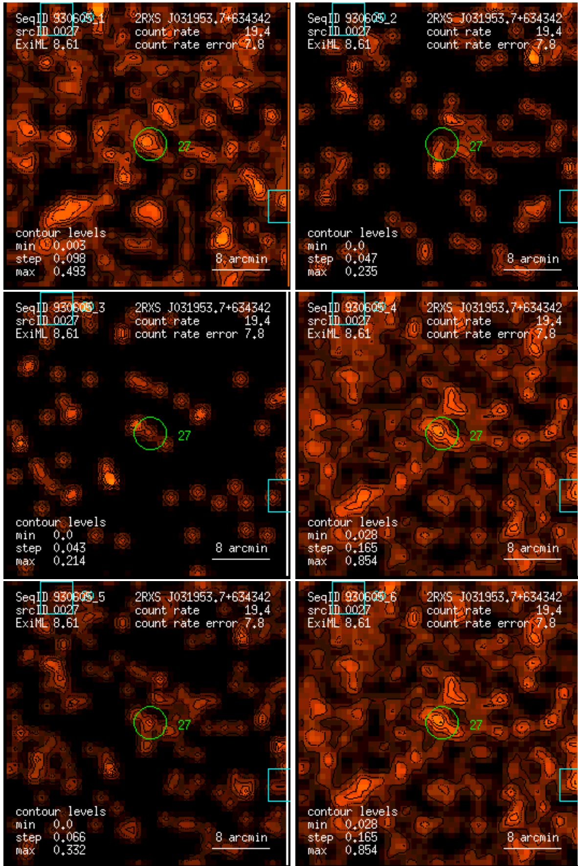
Figure 27: RASS 930605: detection 0027: band rate images, Gaussian filter: (1) PSPC channels 11 – 41, (2) 52 – 90, (3) 91 – 201, (4) 11 – 235, (5) 52 – 201, (6) 11 – 201. Broad band rates in counts/ks. Band rate contour levels in counts/ks/arcmin 2 .
