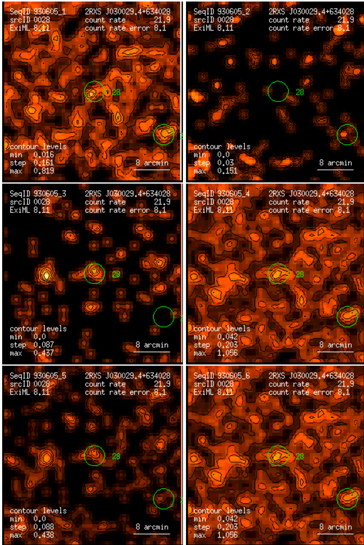
Figure 28: RASS 930605: detection 0028: band rate images, Gaussian filter: (1) PSPC channels 11 – 41, (2) 52 – 90, (3) 91 – 201, (4) 11 – 235, (5) 52 – 201, (6) 11 – 201. Broad band rates in counts/ks. Band rate contour levels in counts/ks/arcmin 2 .
