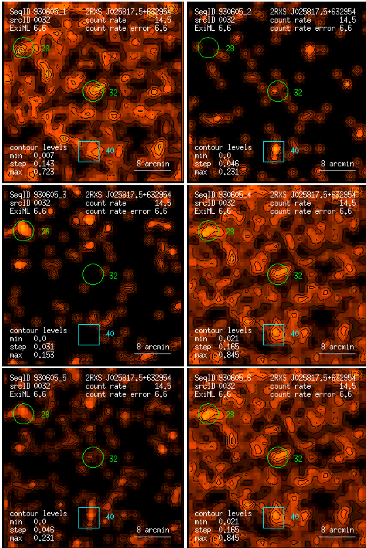
Figure 32: RASS 930605: detection 0032: band rate images, Gaussian filter: (1) PSPC channels 11 – 41, (2) 52 – 90, (3) 91 – 201, (4) 11 – 235, (5) 52 – 201, (6) 11 – 201. Broad band rates in counts/ks. Band rate contour levels in counts/ks/arcmin 2 .
