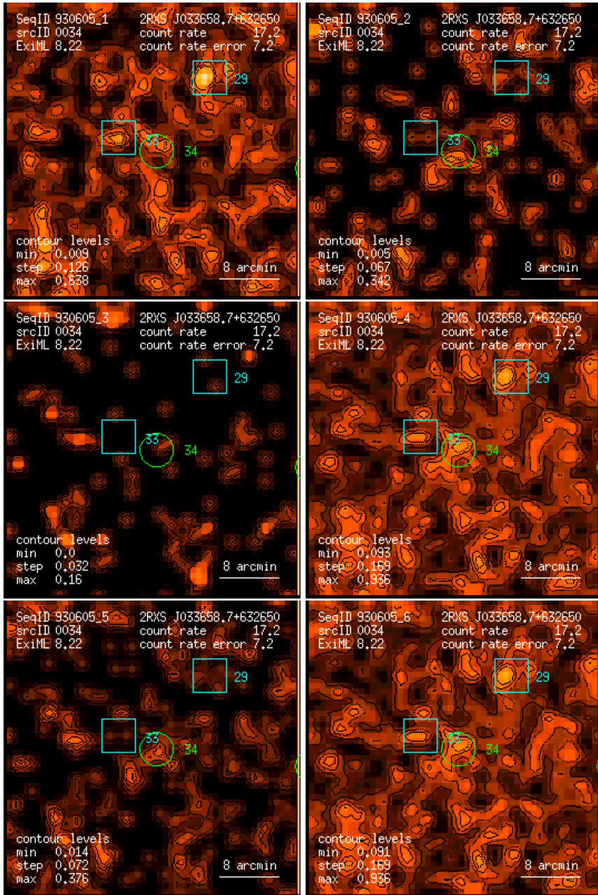
Figure 34: RASS 930605: detection 0034: band rate images, Gaussian filter: (1) PSPC channels 11 – 41, (2) 52 – 90, (3) 91 – 201, (4) 11 – 235, (5) 52 – 201, (6) 11 – 201. Broad band rates in counts/ks. Band rate contour levels in counts/ks/arcmin 2 .
