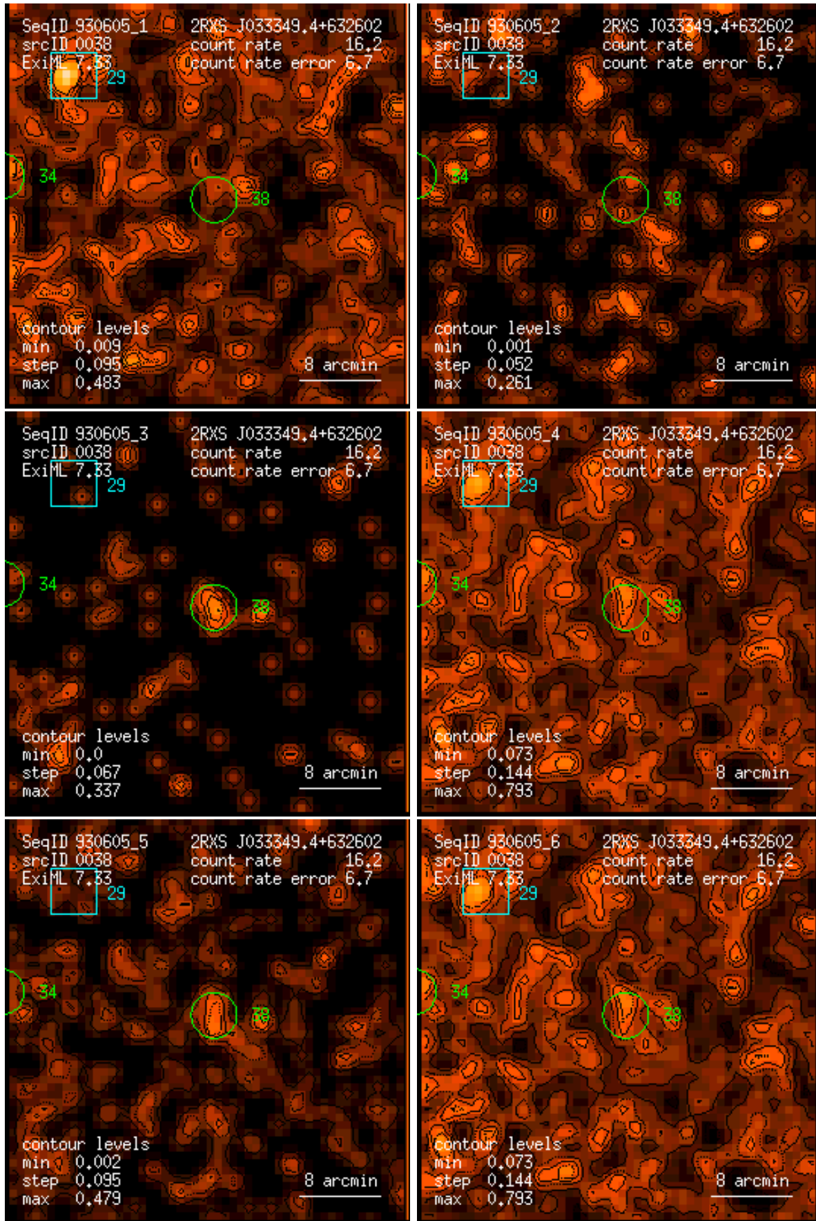
Figure 38: RASS 930605: detection 0038: band rate images, Gaussian filter: (1) PSPC channels 11 – 41, (2) 52 – 90, (3) 91 – 201, (4) 11 – 235, (5) 52 – 201, (6) 11 – 201. Broad band rates in counts/ks. Band rate contour levels in counts/ks/arcmin 2 .
