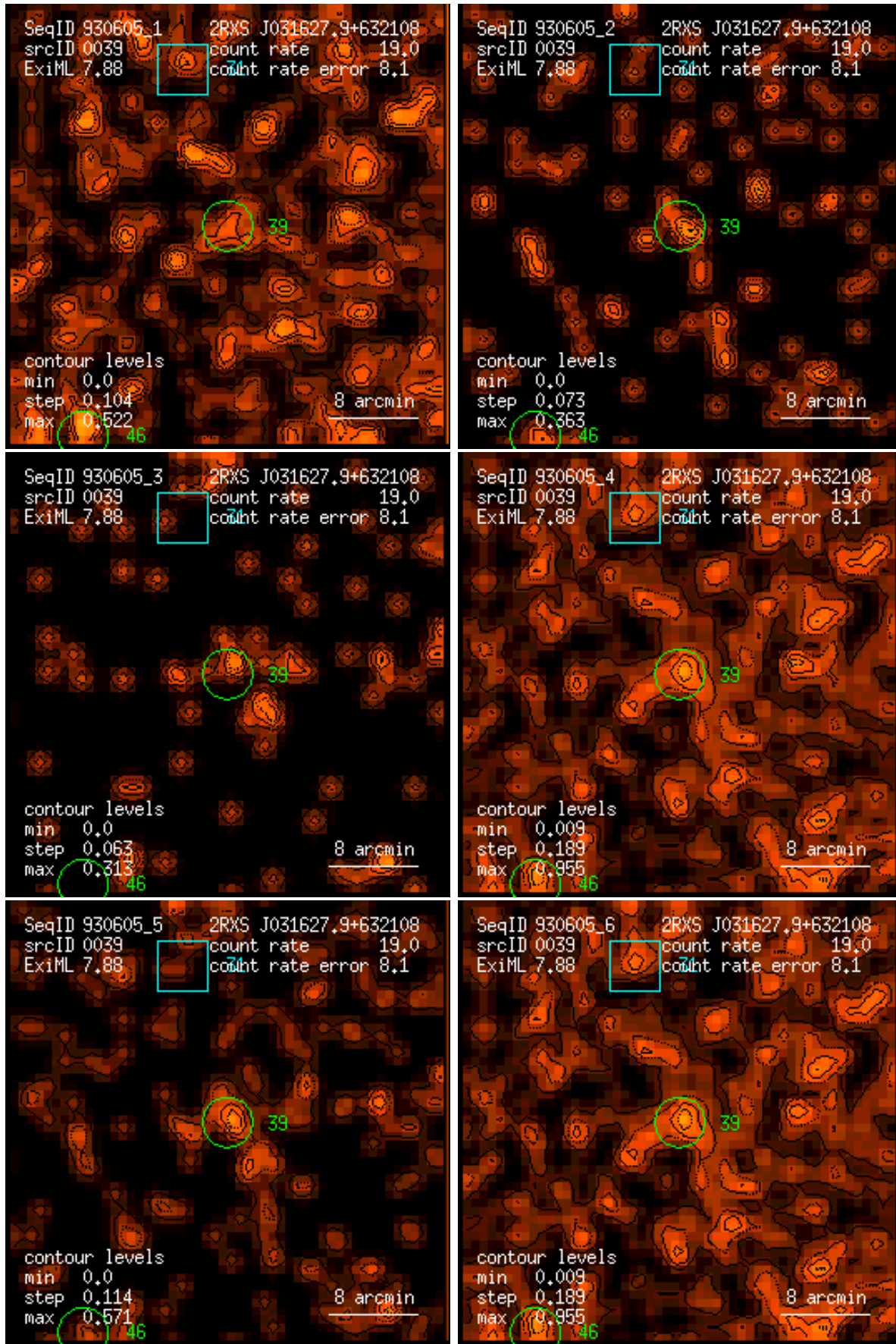
Figure 39: RASS 930605: detection 0039: band rate images, Gaussian filter: (1) PSPC channels 11 – 41, (2) 52 – 90, (3) 91 – 201, (4) 11 – 235, (5) 52 – 201, (6) 11 – 201. Broad band rates in counts/ks. Band rate contour levels in counts/ks/arcmin 2 .
