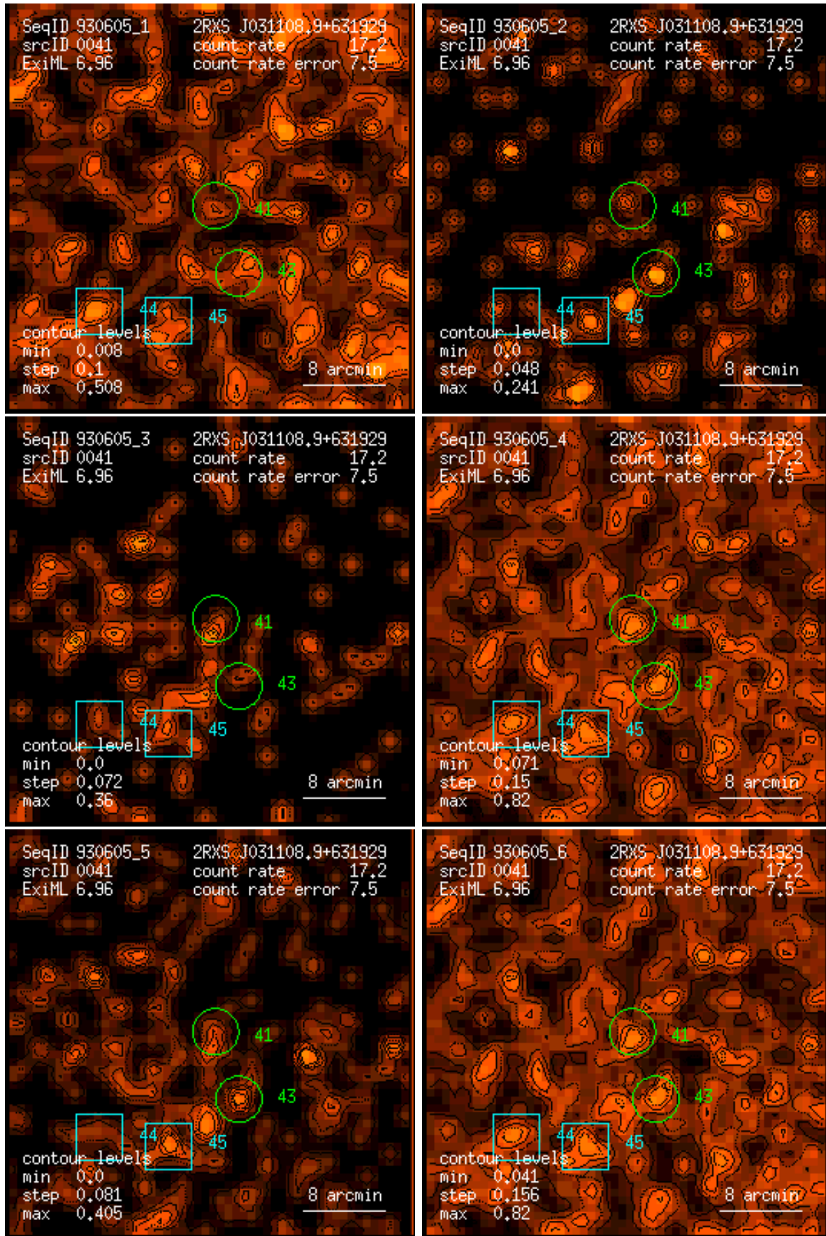
Figure 41: RASS 930605: detection 0041: band rate images, Gaussian filter: (1) PSPC channels 11 – 41, (2) 52 – 90, (3) 91 – 201, (4) 11 – 235, (5) 52 – 201, (6) 11 – 201. Broad band rates in counts/ks. Band rate contour levels in counts/ks/arcmin 2 .
