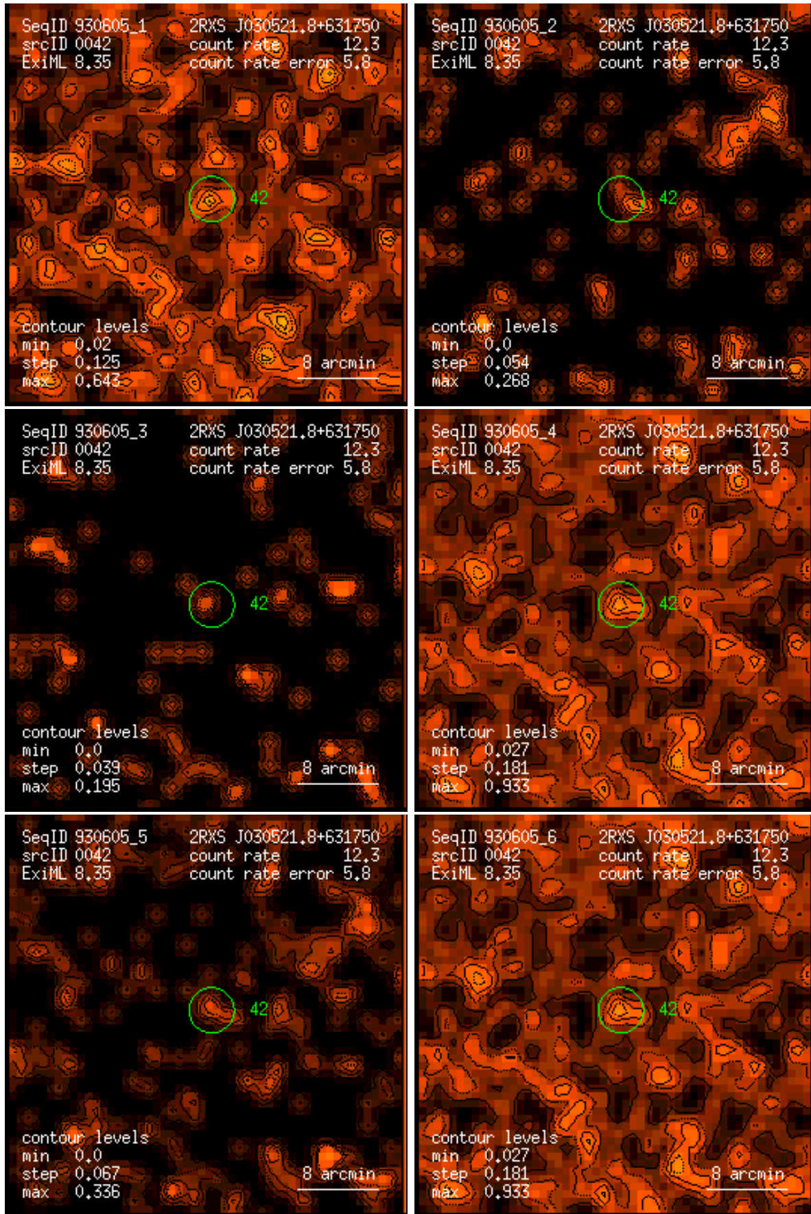
Figure 42: RASS 930605: detection 0042: band rate images, Gaussian filter: (1) PSPC channels 11 – 41, (2) 52 – 90, (3) 91 – 201, (4) 11 – 235, (5) 52 – 201, (6) 11 – 201. Broad band rates in counts/ks. Band rate contour levels in counts/ks/arcmin 2 .
