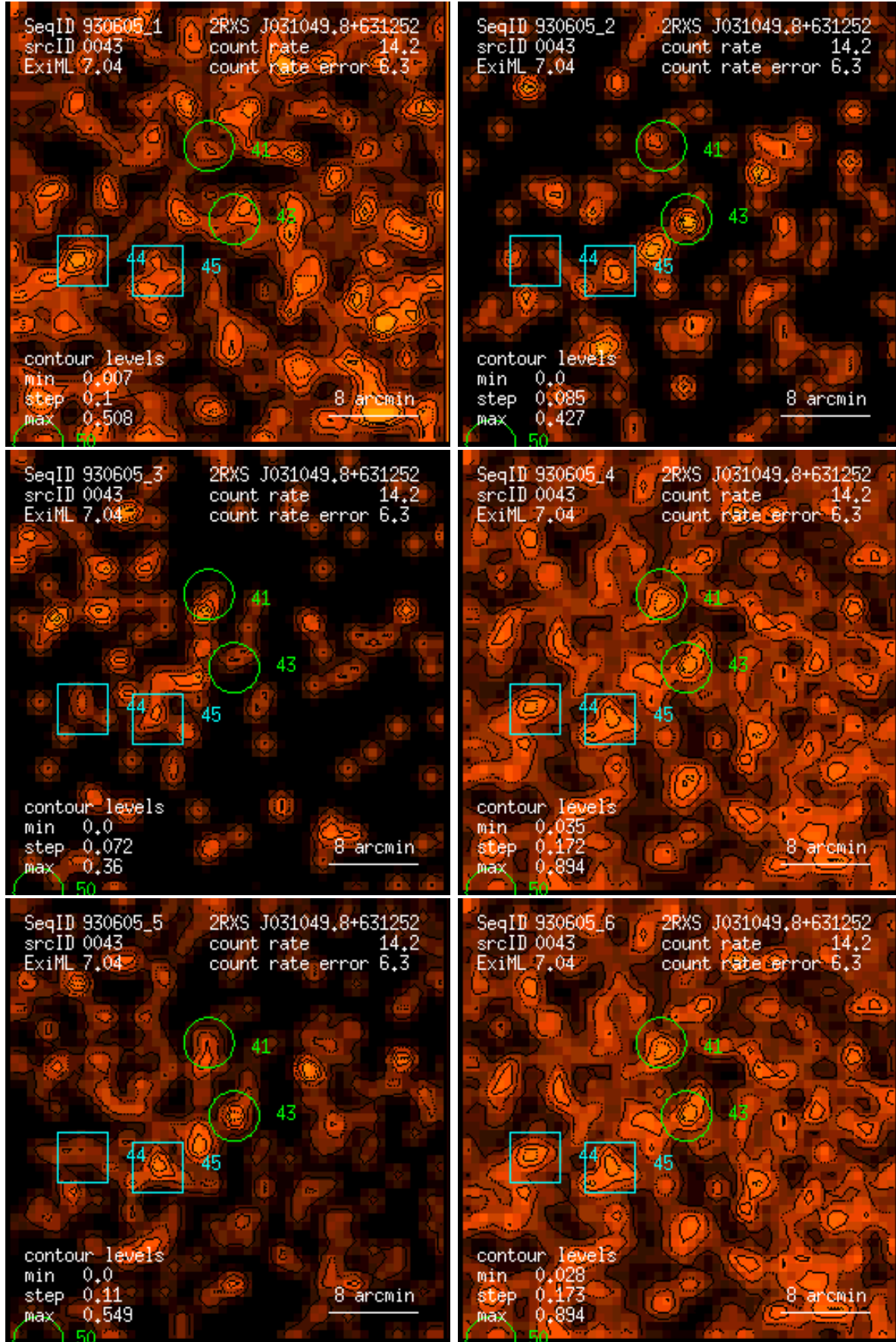
Figure 43: RASS 930605: detection 0043: band rate images, Gaussian filter: (1) PSPC channels 11 – 41, (2) 52 – 90, (3) 91 – 201, (4) 11 – 235, (5) 52 – 201, (6) 11 – 201. Broad band rates in counts/ks. Band rate contour levels in counts/ks/arcmin 2 .
