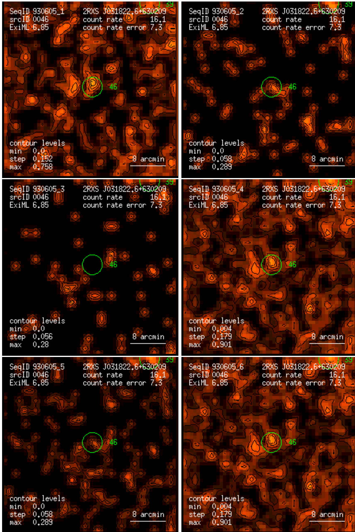
Figure 46: RASS 930605: detection 0046: band rate images, Gaussian filter: (1) PSPC channels 11 – 41, (2) 52 – 90, (3) 91 – 201, (4) 11 – 235, (5) 52 – 201, (6) 11 – 201. Broad band rates in counts/ks. Band rate contour levels in counts/ks/arcmin 2 .
