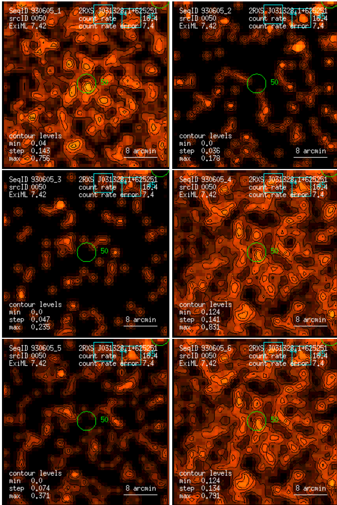
Figure 50: RASS 930605: detection 0050: band rate images, Gaussian filter: (1) PSPC channels 11 – 41, (2) 52 – 90, (3) 91 – 201, (4) 11 – 235, (5) 52 – 201, (6) 11 – 201. Broad band rates in counts/ks. Band rate contour levels in counts/ks/arcmin 2 .
