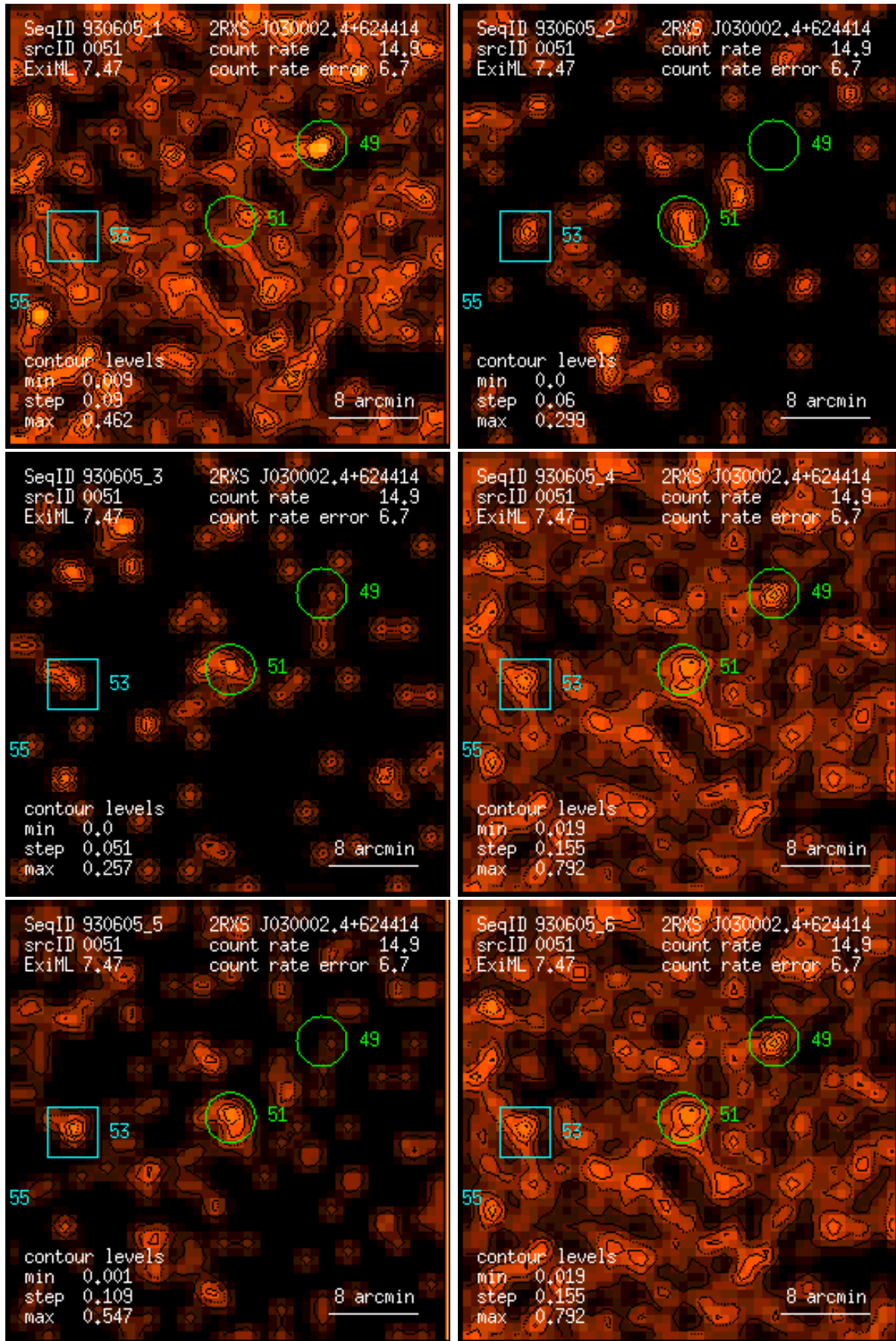
Figure 51: RASS 930605: detection 0051: band rate images, Gaussian filter: (1) PSPC channels 11 – 41, (2) 52 – 90, (3) 91 – 201, (4) 11 – 235, (5) 52 – 201, (6) 11 – 201. Broad band rates in counts/ks. Band rate contour levels in counts/ks/arcmin 2 .
