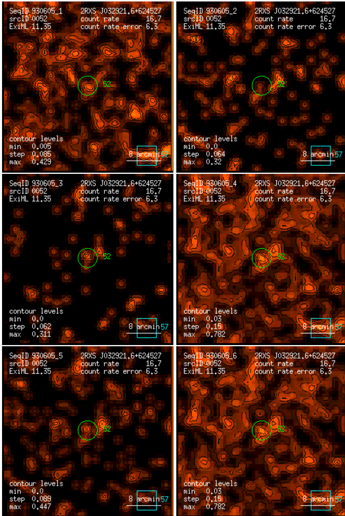
Figure 52: RASS 930605: detection 0052: band rate images, Gaussian filter: (1) PSPC channels 11 – 41, (2) 52 – 90, (3) 91 – 201, (4) 11 – 235, (5) 52 – 201, (6) 11 – 201. Broad band rates in counts/ks. Band rate contour levels in counts/ks/arcmin 2 .
