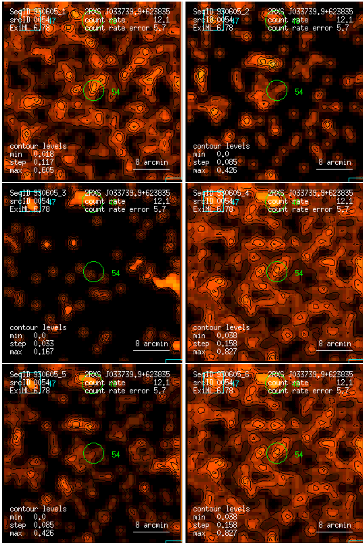
Figure 54: RASS 930605: detection 0054: band rate images, Gaussian filter: (1) PSPC channels 11 – 41, (2) 52 – 90, (3) 91 – 201, (4) 11 – 235, (5) 52 – 201, (6) 11 – 201. Broad band rates in counts/ks. Band rate contour levels in counts/ks/arcmin 2 .
