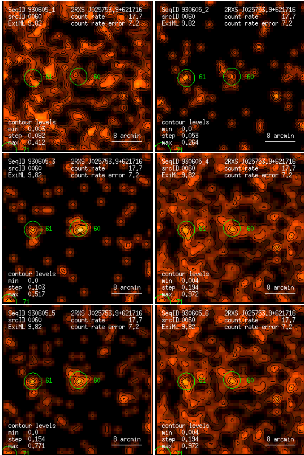
Figure 60: RASS 930605: detection 0060: band rate images, Gaussian filter: (1) PSPC channels 11 – 41, (2) 52 – 90, (3) 91 – 201, (4) 11 – 235, (5) 52 – 201, (6) 11 – 201. Broad band rates in counts/ks. Band rate contour levels in counts/ks/arcmin 2 .
