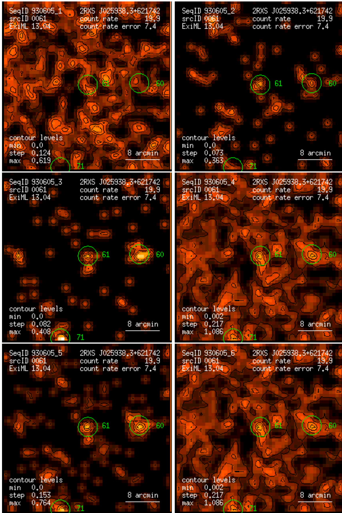
Figure 61: RASS 930605: detection 0061: band rate images, Gaussian filter: (1) PSPC channels 11 – 41, (2) 52 – 90, (3) 91 – 201, (4) 11 – 235, (5) 52 – 201, (6) 11 – 201. Broad band rates in counts/ks. Band rate contour levels in counts/ks/arcmin 2 .
