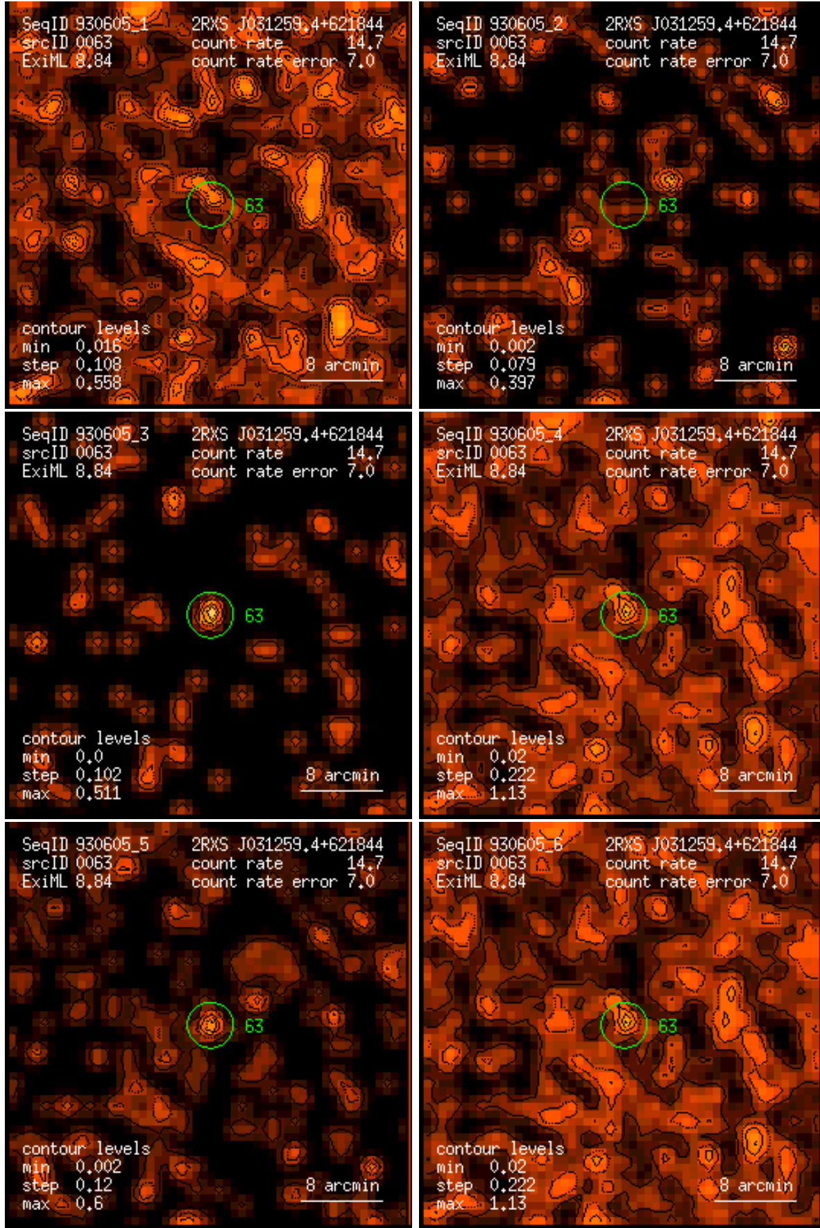
Figure 63: RASS 930605: detection 0063: band rate images, Gaussian filter: (1) PSPC channels 11 – 41, (2) 52 – 90, (3) 91 – 201, (4) 11 – 235, (5) 52 – 201, (6) 11 – 201. Broad band rates in counts/ks. Band rate contour levels in counts/ks/arcmin 2 .
