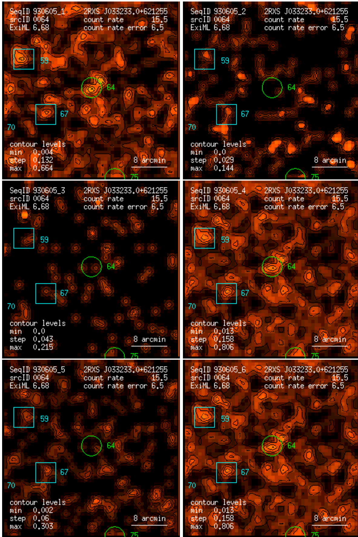
Figure 64: RASS 930605: detection 0064: band rate images, Gaussian filter: (1) PSPC channels 11 – 41, (2) 52 – 90, (3) 91 – 201, (4) 11 – 235, (5) 52 – 201, (6) 11 – 201. Broad band rates in counts/ks. Band rate contour levels in counts/ks/arcmin 2 .
