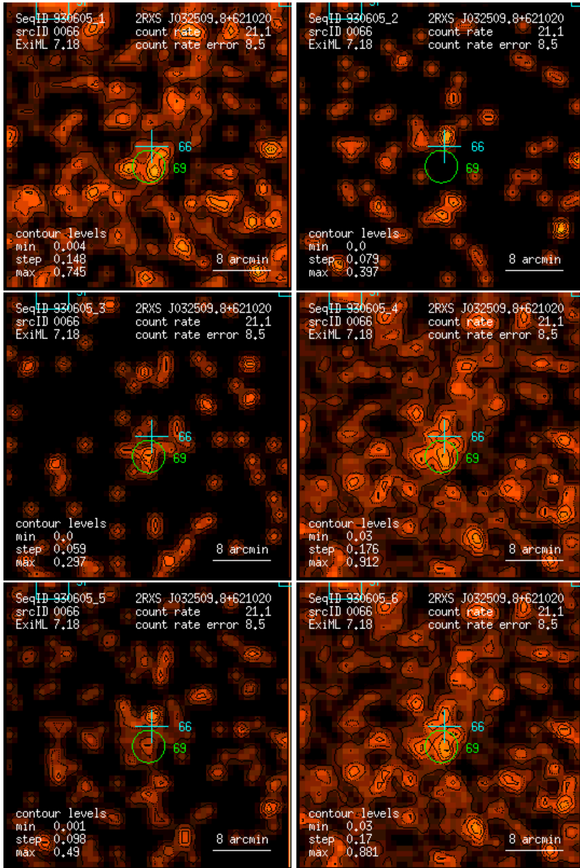
Figure 66: RASS 930605: detection 0066: band rate images, Gaussian filter: (1) PSPC channels 11 – 41, (2) 52 – 90, (3) 91 – 201, (4) 11 – 235, (5) 52 – 201, (6) 11 – 201. Broad band rates in counts/ks. Band rate contour levels in counts/ks/arcmin 2 .
