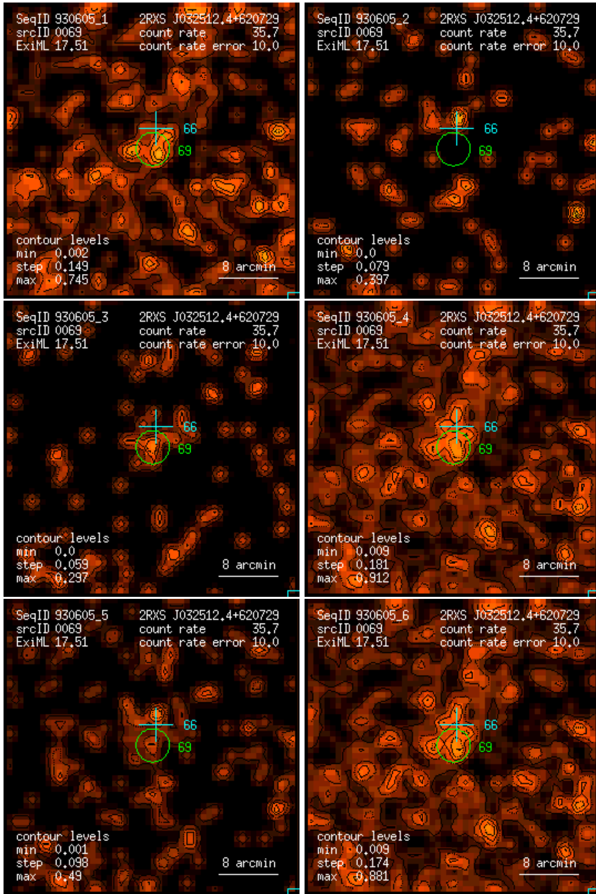
Figure 69: RASS 930605: detection 0069: band rate images, Gaussian filter: (1) PSPC channels 11 – 41, (2) 52 – 90, (3) 91 – 201, (4) 11 – 235, (5) 52 – 201, (6) 11 – 201. Broad band rates in counts/ks. Band rate contour levels in counts/ks/arcmin 2 .
