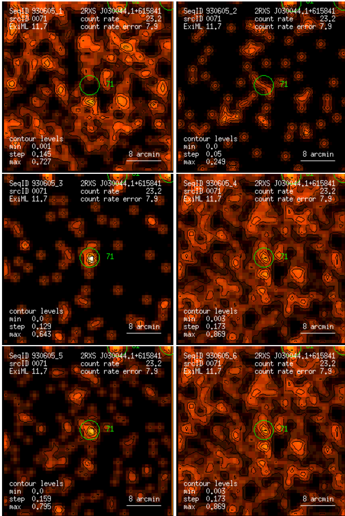
Figure 71: RASS 930605: detection 0071: band rate images, Gaussian filter: (1) PSPC channels 11 – 41, (2) 52 – 90, (3) 91 – 201, (4) 11 – 235, (5) 52 – 201, (6) 11 – 201. Broad band rates in counts/ks. Band rate contour levels in counts/ks/arcmin 2 .
