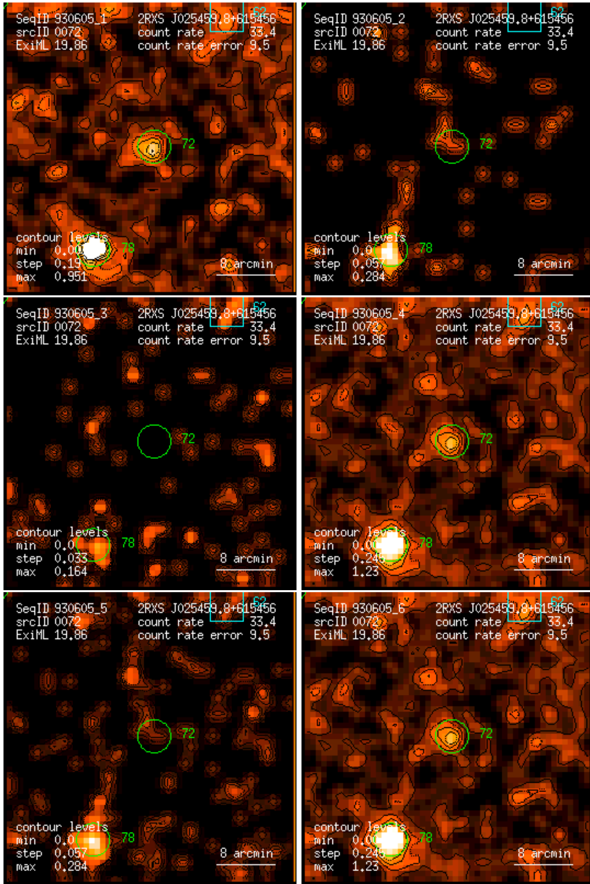
Figure 72: RASS 930605: detection 0072: band rate images, Gaussian filter: (1) PSPC channels 11 – 41, (2) 52 – 90, (3) 91 – 201, (4) 11 – 235, (5) 52 – 201, (6) 11 – 201. Broad band rates in counts/ks. Band rate contour levels in counts/ks/arcmin 2 .
