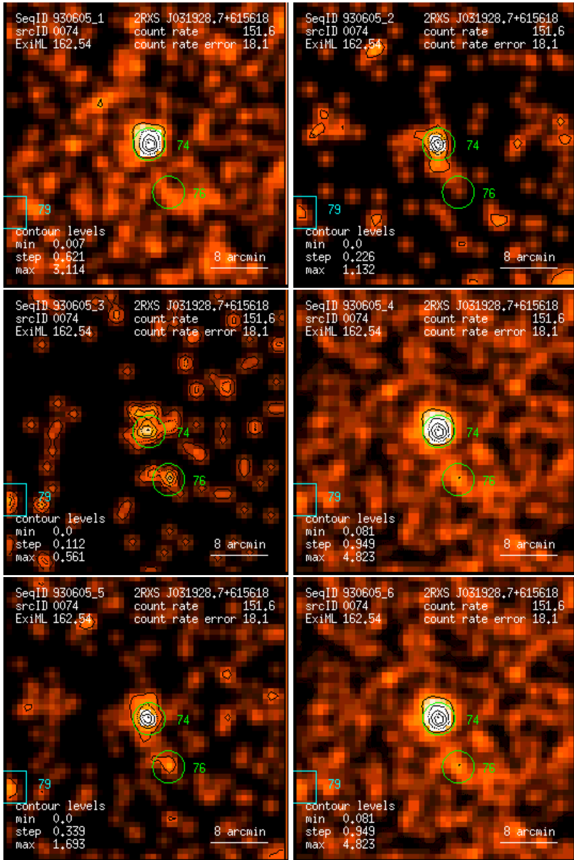
Figure 74: RASS 930605: detection 0074: band rate images, Gaussian filter: (1) PSPC channels 11 – 41, (2) 52 – 90, (3) 91 – 201, (4) 11 – 235, (5) 52 – 201, (6) 11 – 201. Broad band rates in counts/ks. Band rate contour levels in counts/ks/arcmin 2 .
