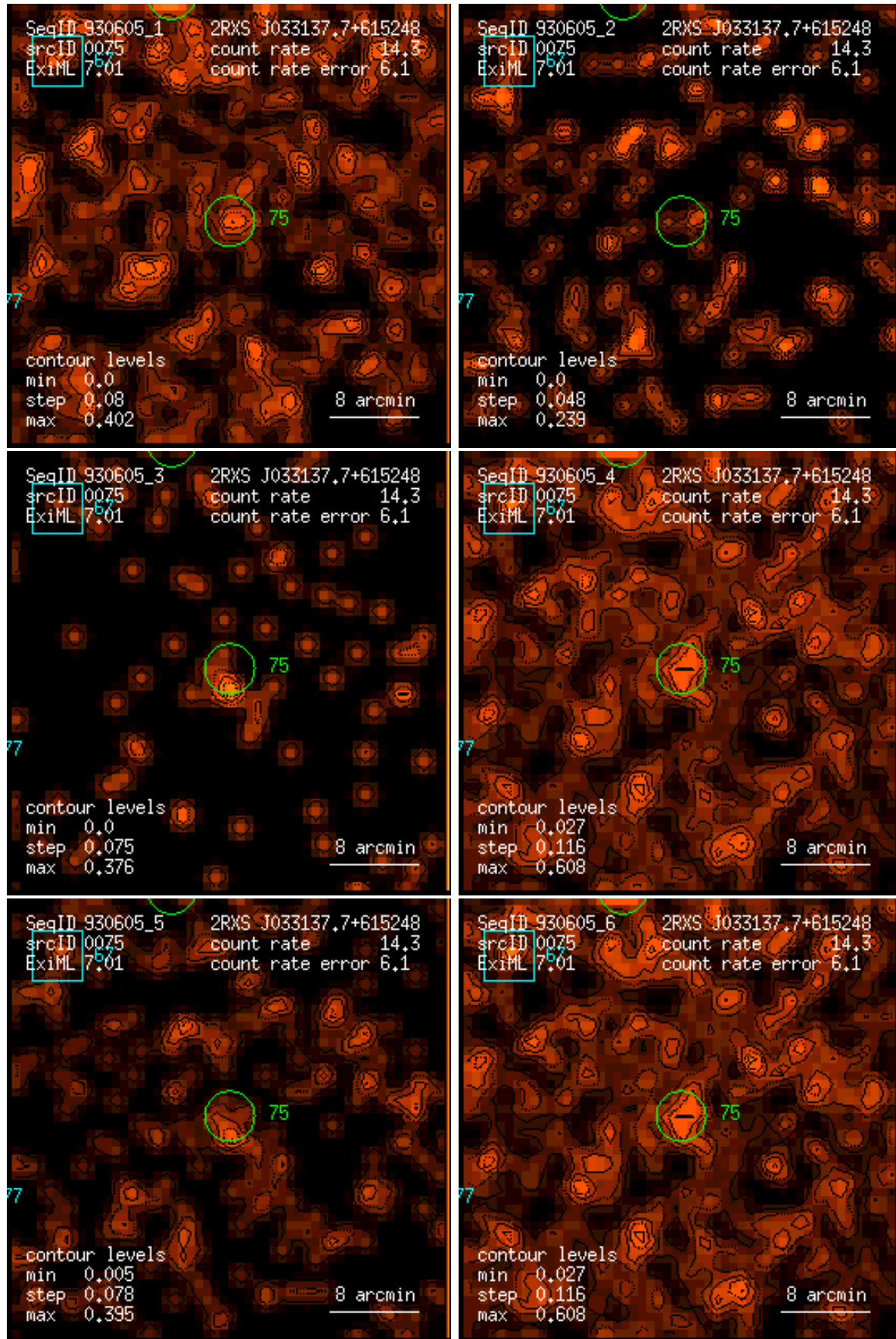
Figure 75: RASS 930605: detection 0075: band rate images, Gaussian filter: (1) PSPC channels 11 – 41, (2) 52 – 90, (3) 91 – 201, (4) 11 – 235, (5) 52 – 201, (6) 11 – 201. Broad band rates in counts/ks. Band rate contour levels in counts/ks/arcmin 2 .
